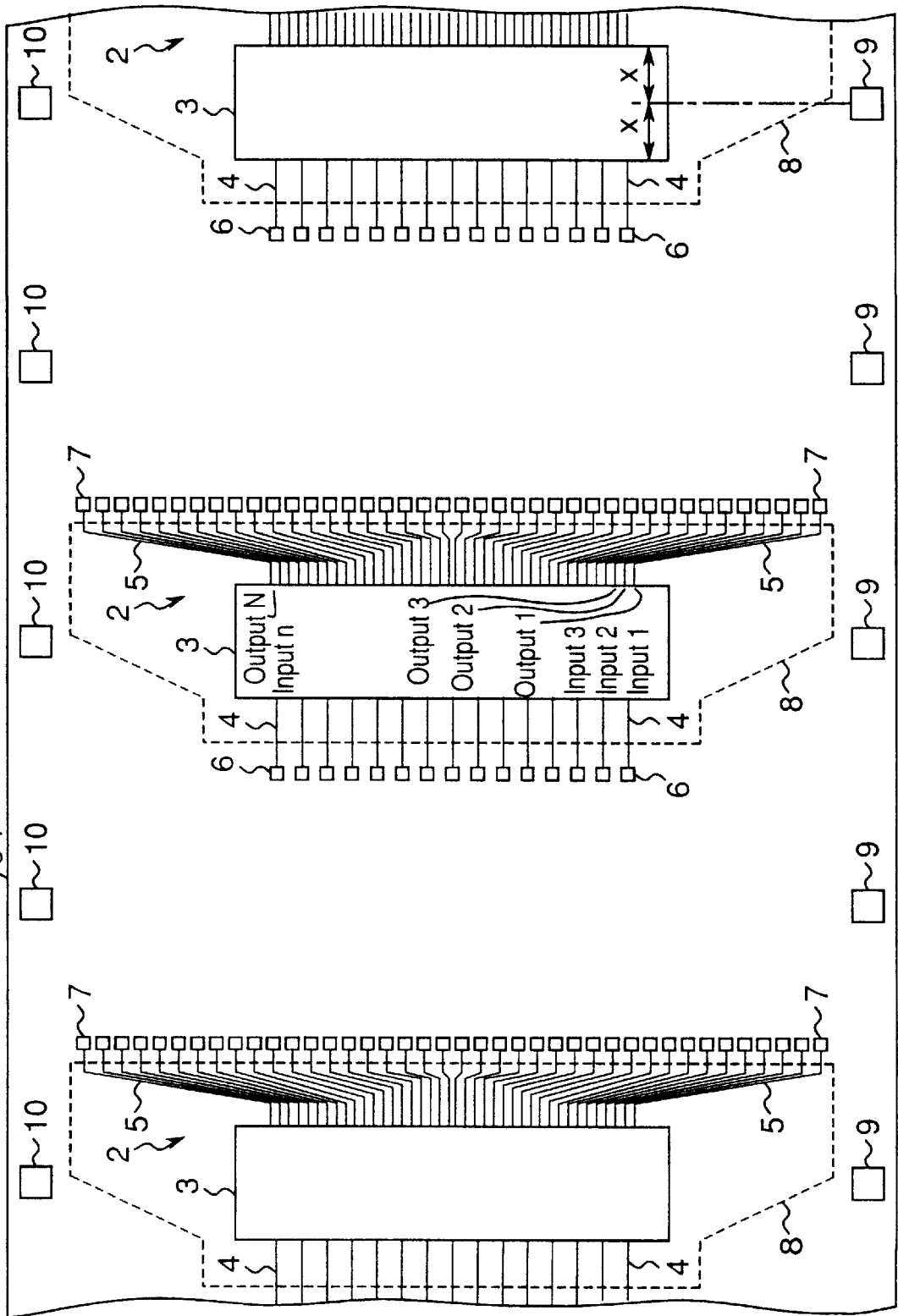
Fig. 10 PRIOR ART
