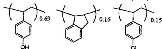
Polymer 2
