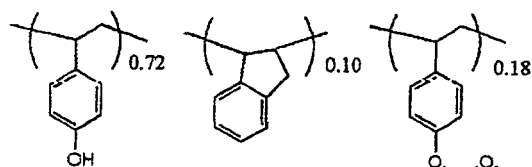
Polymer 1
