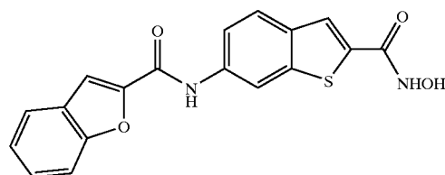
COMPOUND 112
