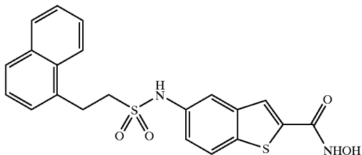
COMPOUND 8
