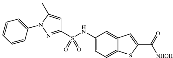
COMPOUND 35
