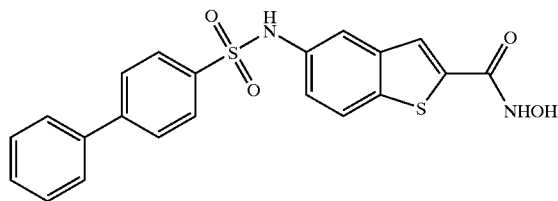
COMPOUND 71
