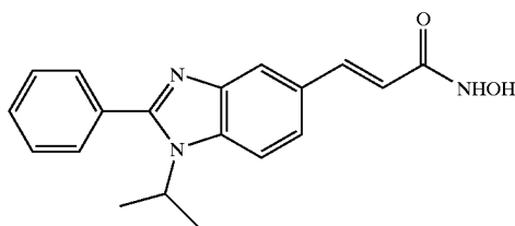
COMPOUND 102
