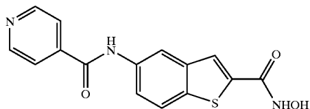
COMPOUND 32
