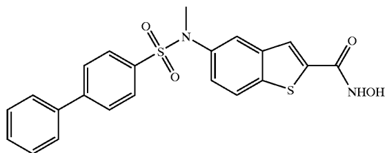
COMPOUND 72
