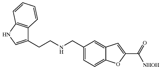
COMPOUND 53
