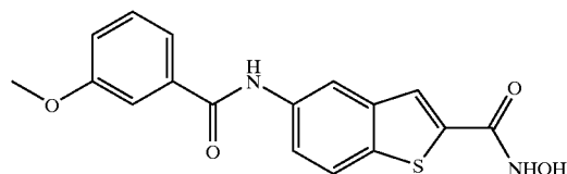
COMPOUND 18
