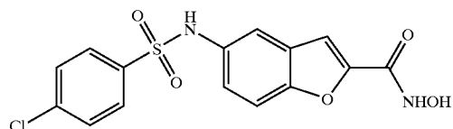
COMPOUND 81
