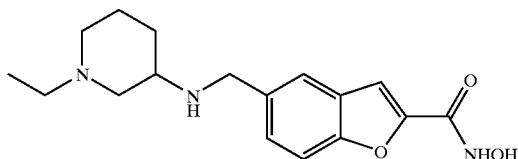
COMPOUND 60
