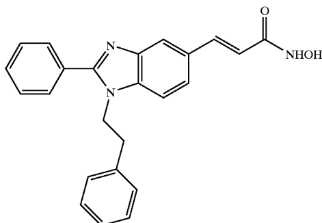
COMPOUND 100
