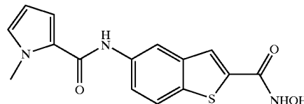
1-Methyl-1H-pyrrole-2-carboxylic Acid (2-hydroxycarbamoyl-benzo[b]thiophen-5-yl)-amide
