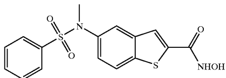
COMPOUND 77
