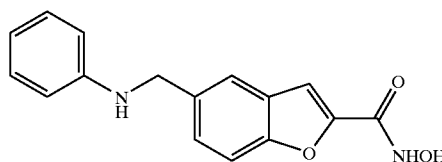
COMPOUND 52
