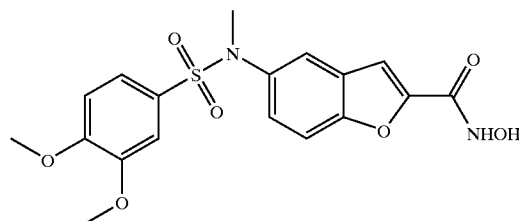
COMPOUND 104
