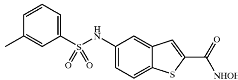
COMPOUND 2
