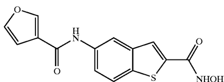
Furan-3-carboxylic Acid (2-hydroxycarbamoyl-benzo[b]thiophen-5-yl)-amide
