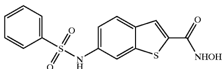
COMPOUND 107
