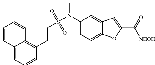
COMPOUND 86
