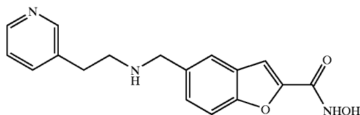
COMPOUND 58
