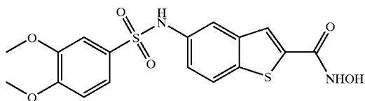
5-(3,4-Dimethoxy-benzenesulfonylamino)-benzo[b]thiophene-2-carboxylic Acid Hydroxyamide
