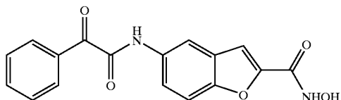
COMPOUND 84
