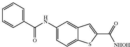
COMPOUND 15
