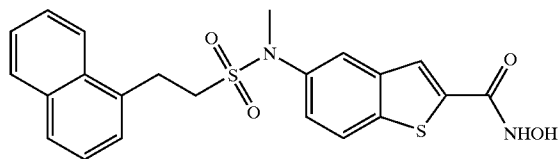
COMPOUND 73
