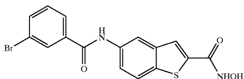
COMPOUND 20
