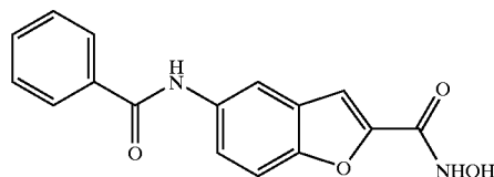
COMPOUND 80
