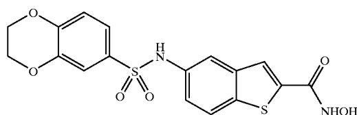
COMPOUND 25
