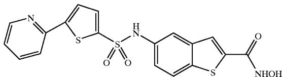
COMPOUND 38
