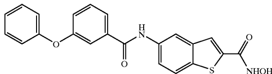
COMPOUND 23
