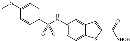
COMPOUND 12
