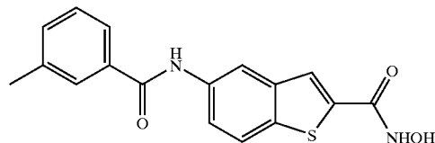
COMPOUND 16
