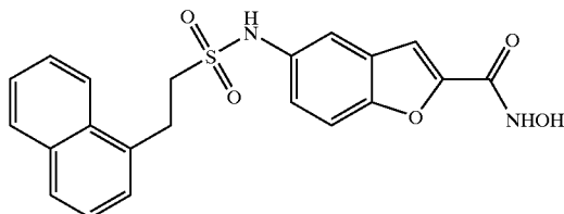
COMPOUND 82
