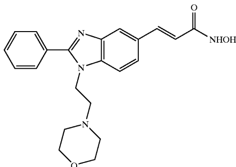
COMPOUND 101
