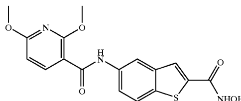
COMPOUND 44
