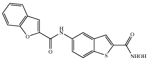
COMPOUND 42
