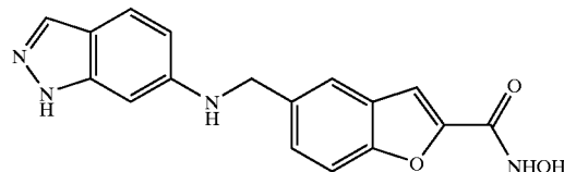
COMPOUND 66
