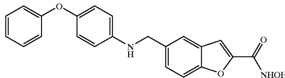
COMPOUND 65
