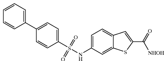
COMPOUND 105
