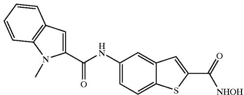
COMPOUND 49
