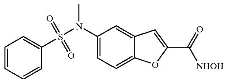
COMPOUND 88
