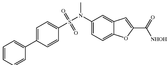
COMPOUND 87
