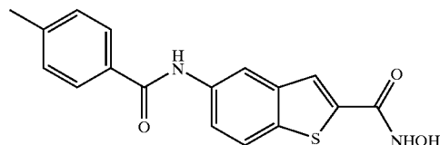
COMPOUND 17
