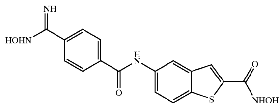
COMPOUND 30
