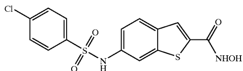
COMPOUND 108
