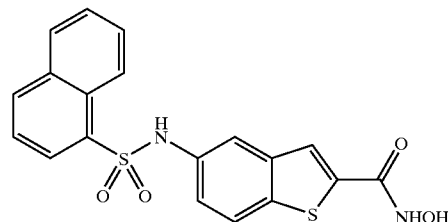
COMPOUND 9
