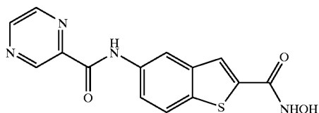
COMPOUND 46
