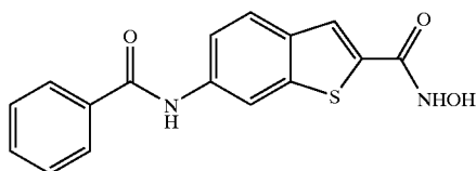
COMPOUND 106
