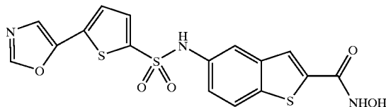
COMPOUND 37
