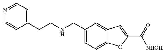
COMPOUND 59
