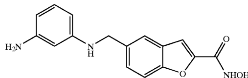
COMPOUND 64
