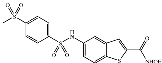
COMPOUND 26
