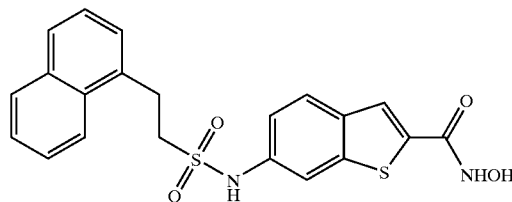
COMPOUND 109
