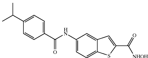
COMPOUND 47
