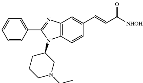
COMPOUND 90
