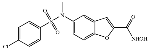
COMPOUND 85
