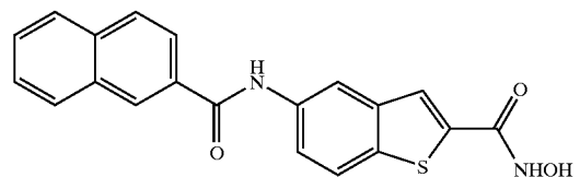
COMPOUND 31
