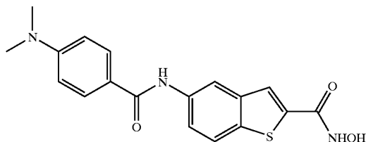
COMPOUND 28
