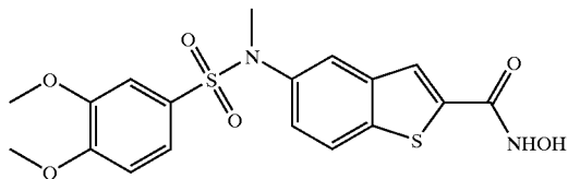
COMPOUND 74
