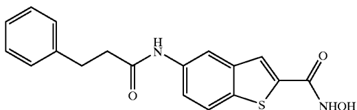
COMPOUND 33
