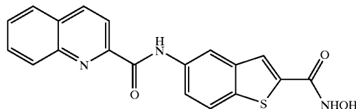
COMPOUND 45
