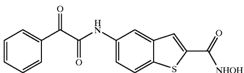
COMPOUND 48
