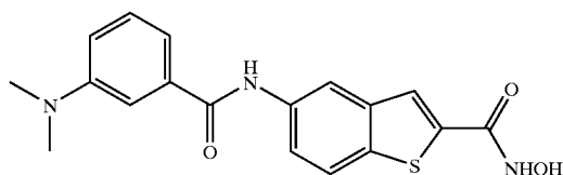
COMPOUND 27
