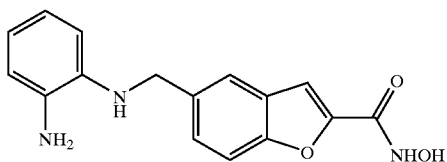
COMPOUND 63
