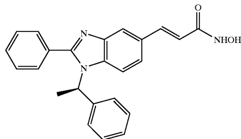
COMPOUND 103
