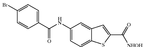
COMPOUND 21
