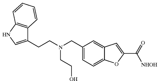
COMPOUND 54
