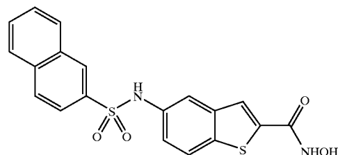
COMPOUND 10
