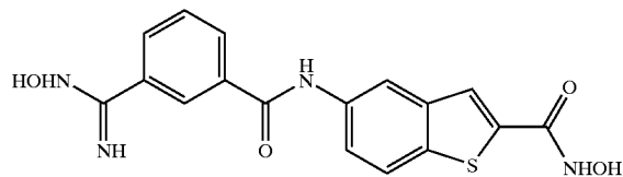
COMPOUND 29
