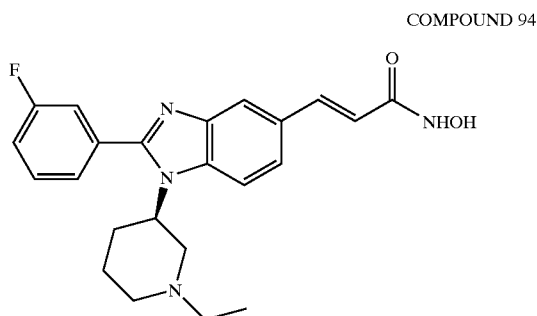
(R)-3-[1-(1-Ethyl-piperidin-3-yl)-2-(3-fluoro-phenyl)-1H-benzoimidazol-5-yl]-N-hydroxy-acrylamide
