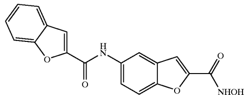
COMPOUND 78
