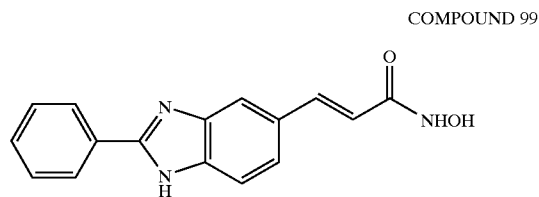
N-Hydroxy-3-(2-phenyl-1H-benzoimidazol-5-yl)-acrylamide
