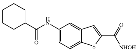
COMPOUND 13
