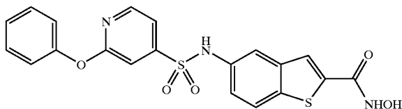
COMPOUND 36
