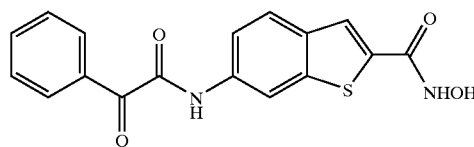
COMPOUND 111
