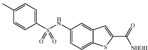
COMPOUND 1
