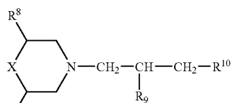
(TRIDEMORPH)
