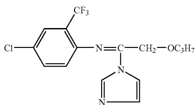
(TRIFLUMIZOLE)
