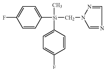
(FLUSILAZOLE)
