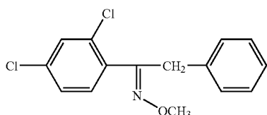
(PYRIFENOX)
