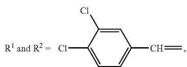
(DINICONAZOLE)
