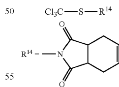
(CAPTAN)
