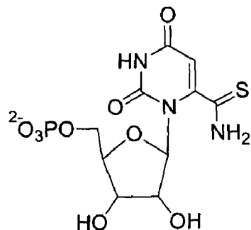
6-Thiocarboxamido UMP (13)
