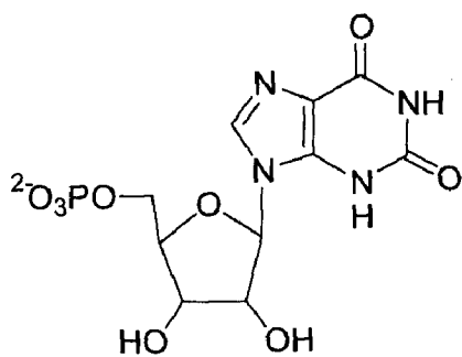
XMP (12)
