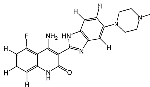
Tautomer Ib
