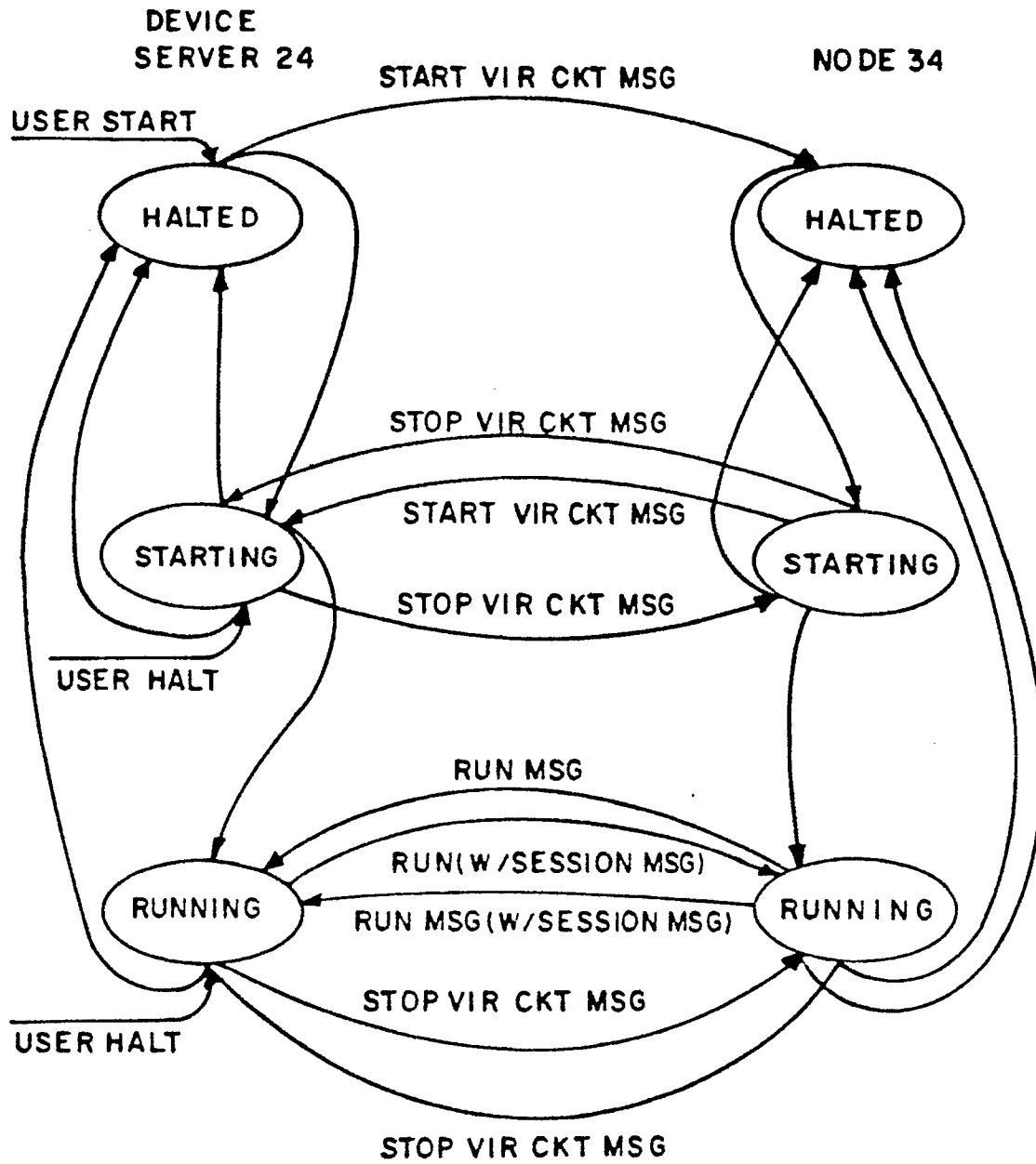
VIRTUAL CIRCUIT STATE DIAGRAM
