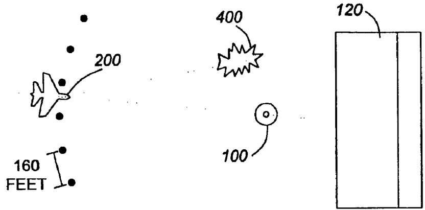
TOP VIEW FIG. 4A
