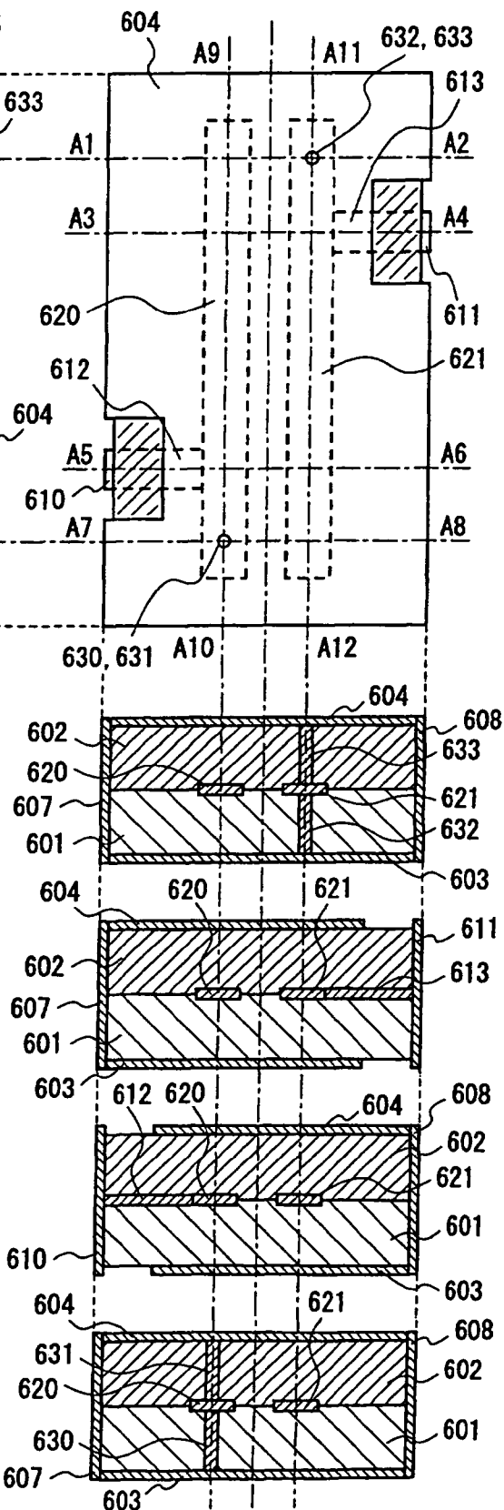
Fig.6 (c) PRIOR ART
