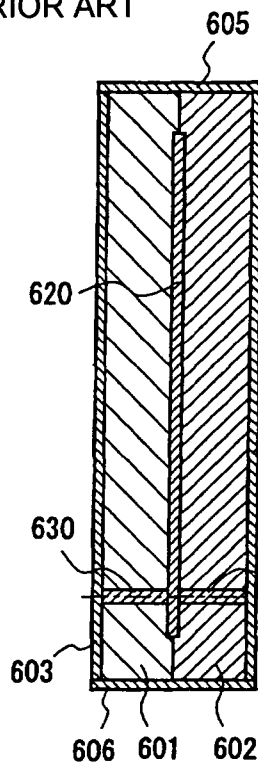
Fig.6 (a) PRIOR ART
