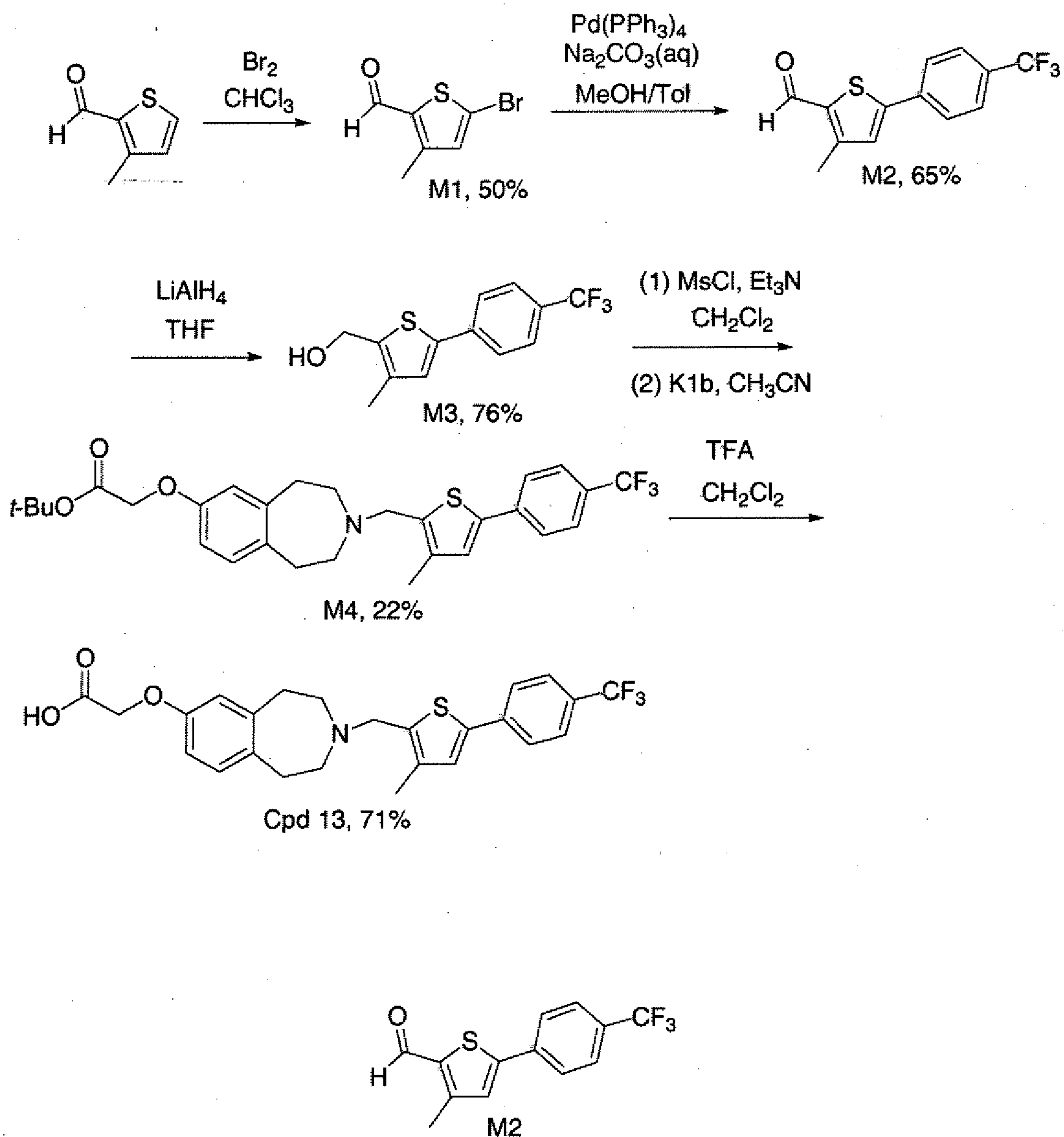
3-Methyl-5-(4-trifluoromethyl-phenyl)-thiophene-2-carbaldehyde
