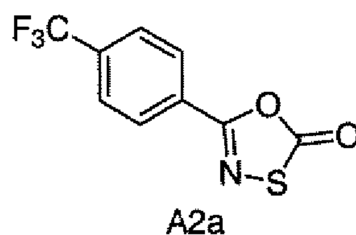
5-(4-Trifluoromethyl-phenyl)-[1,3,4]oxathiazol-2-one
