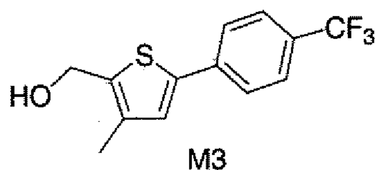
[3-Methyl-5-(4-trifluoromethyl-phenyl)-thiophen-2-yl]-methanol
