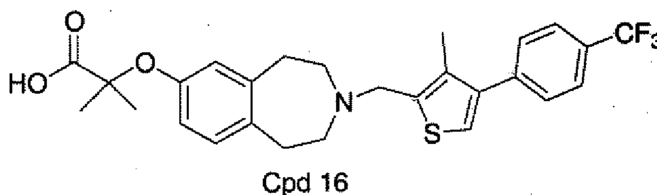
2-Methyl-2-{3-[3-methyl-4-(4-trifluoromethyl-phenyl)-thiophen-2-ylmethyl]-2,3,4,5-tetrahydro-1H-benzo[d]azepin-7-yloxy}-propionic acid
