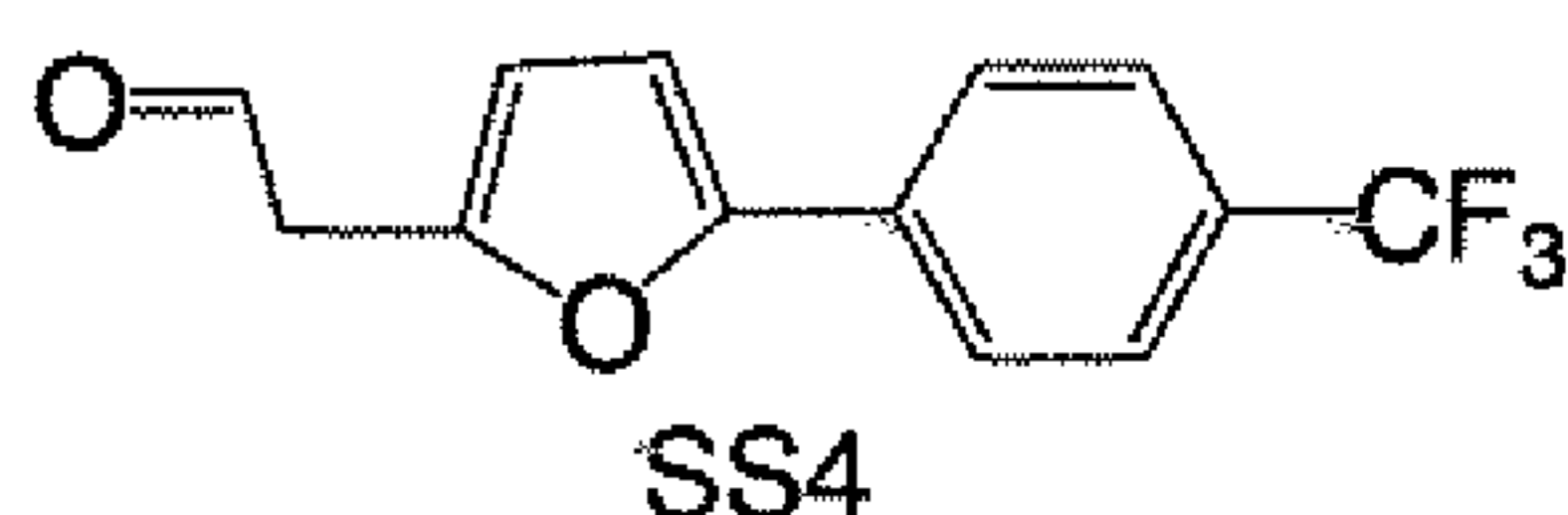
[5-(4-Trifluoromethyl-phenyl)-furan-2-yl]-acetaldehyde
