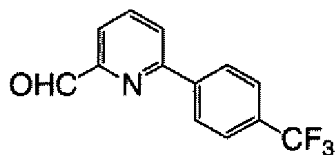
6-(4-Trifluoromethyl-phenyl)-pyridine-2-carbaldehyde
