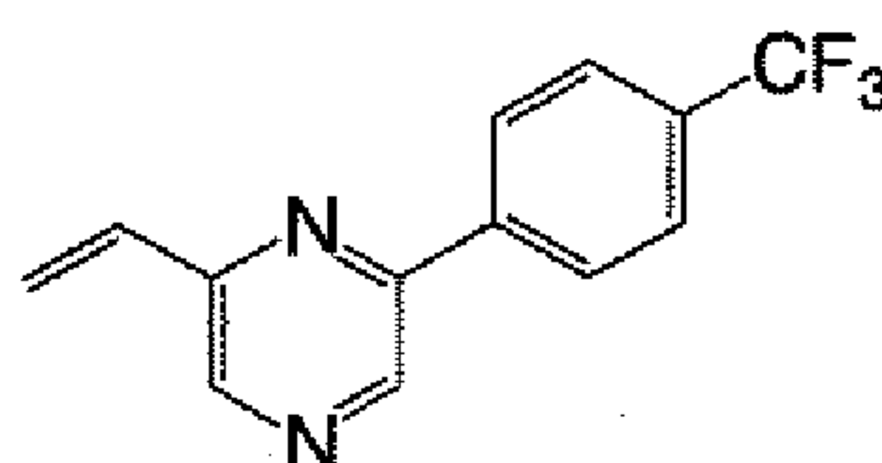
2-(4-Trifluoromethyl-phenyl)-6-vinyl-pyrazine
