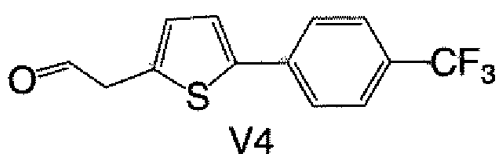
[5-(4-Trifluoromethyl-phenyl)-thiophen-2-yl]-acetaldehyde
