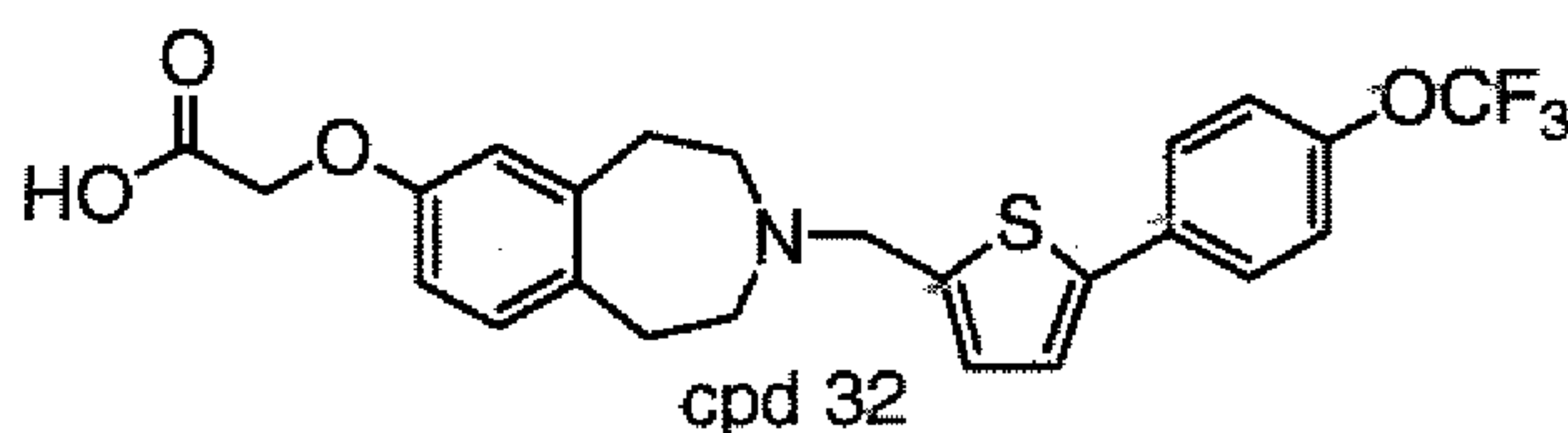
{3-[5-(4-Trifluoromethoxy-phenyl)-thiophen-2-ylmethyl]-2,3,4,5-tetrahydro-1H-benzo[d]azepin-7-yloxy}-acetic acid
