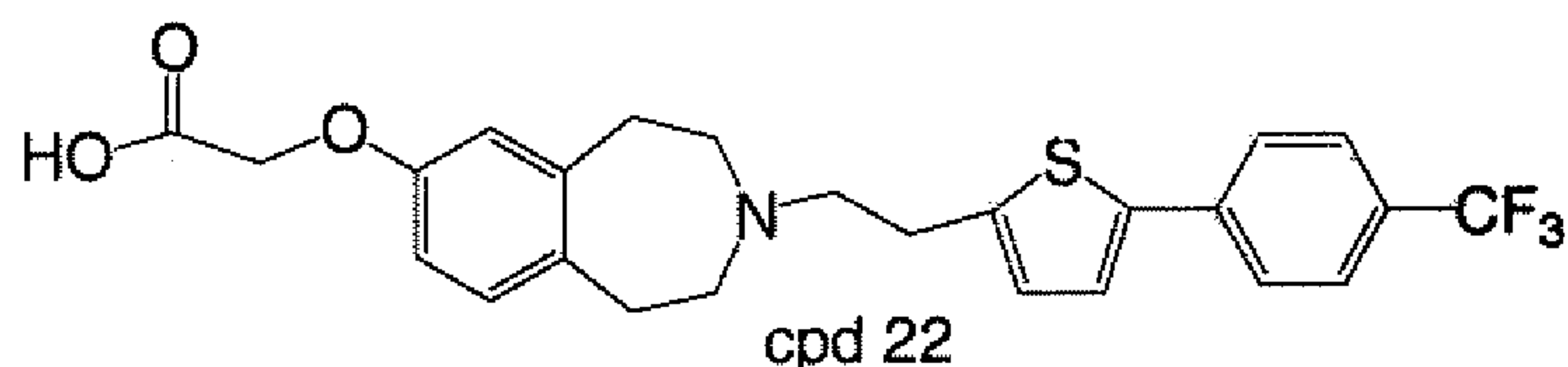
(3-{2-[5-(4-Trifluoromethyl-phenyl)-thiophen-2-yl]-ethyl}-2,3,4,5-tetrahydro-1H-benzo[d]azepin-7-yloxy)-acetic acid
