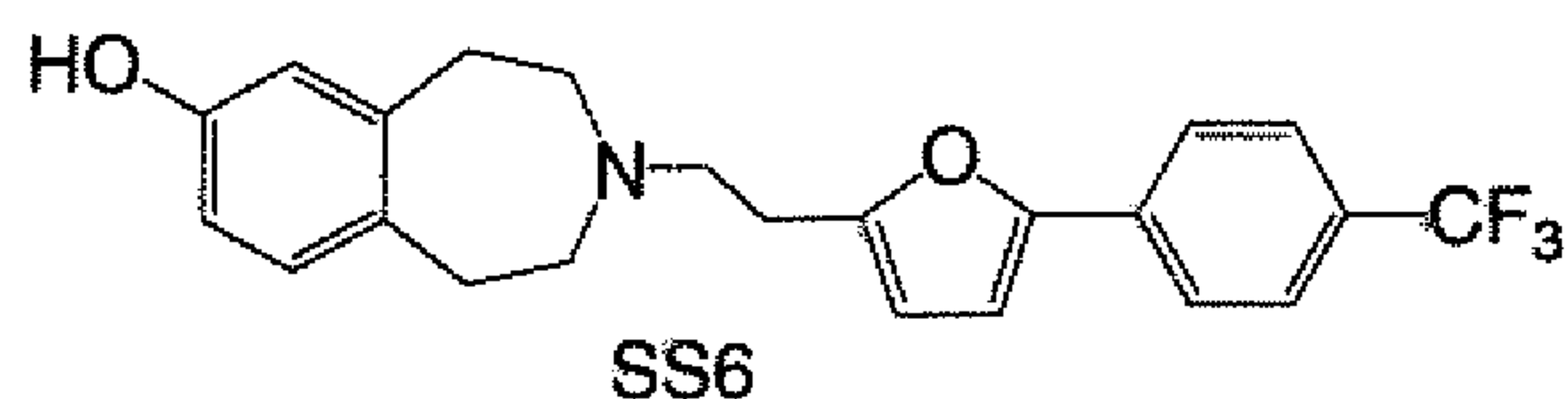
3-{2-[5-(4-Trifluoromethyl-phenyl)-furan-2-yl]-ethyl}-2,3,4,5-tetrahydro-1H-benzo[d]azepin-7-ol
