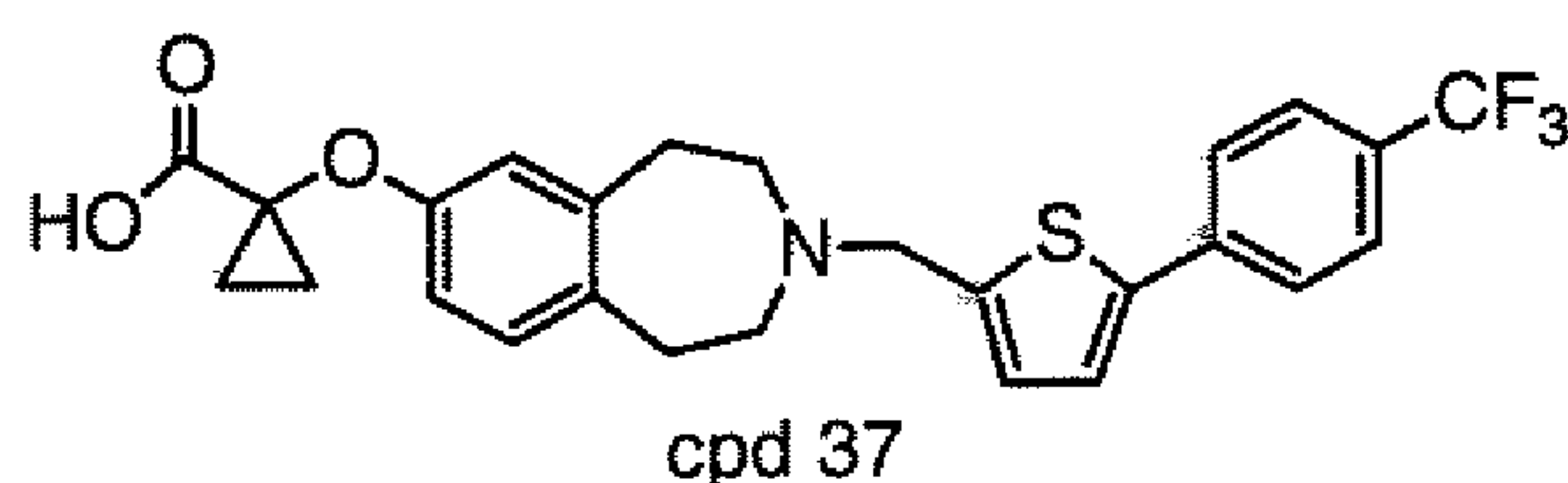
1-{3-[5-(4-Trifluoromethyl-phenyl)-thiophen-2-ylmethyl]-2,3,4,5-tetrahydro-1H-benzo[d]azepin-7-yloxy}-cyclopropanecarboxylic acid
