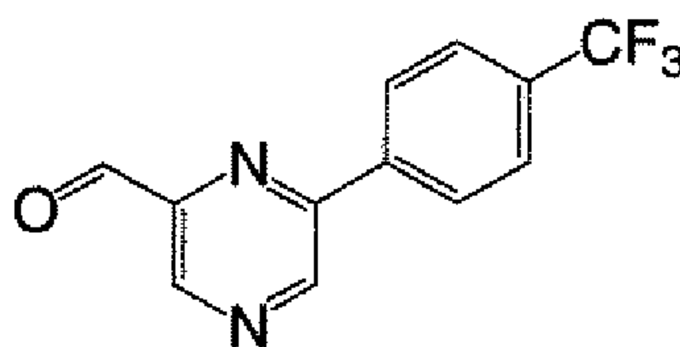
6-(4-Trifluoromethyl-phenyl)-pyrazine-2-carbaldehyde
