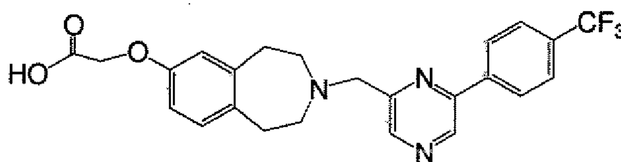
{3-[6-(4-Trifluoromethyl-phenyl)-pyrazin-2-ylmethyl]-2,3,4,5-tetrahydro-1H-benzo[d]azepin-7-yloxy}-acetic acid
