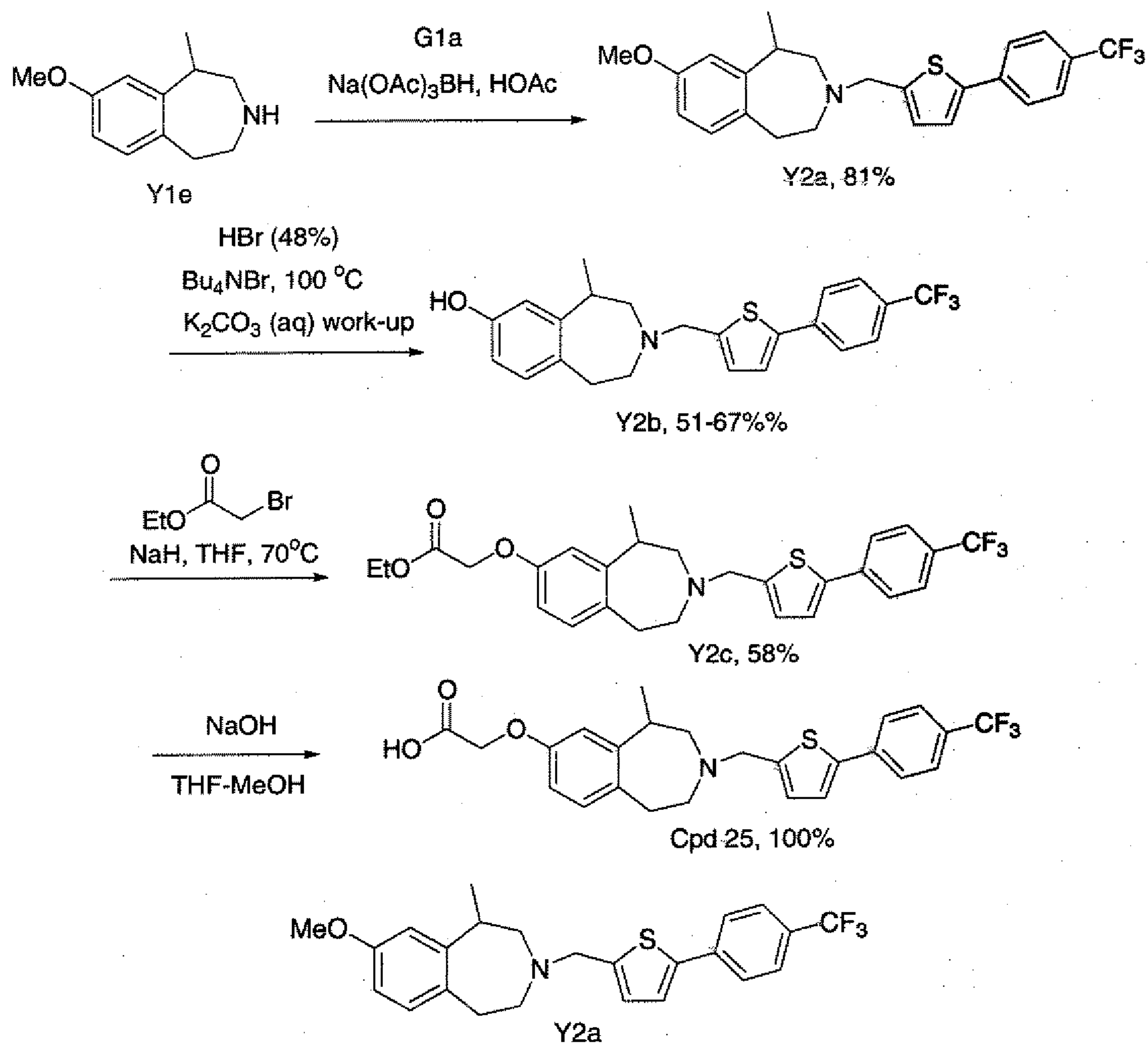
8-Methoxy-1-methyl-3-[5-(4-trifluoromethyl-phenyl)-thiophen-2-ylmethyl]-2,3,4,5-tetrahydro-1H-benzo[d]azepine
