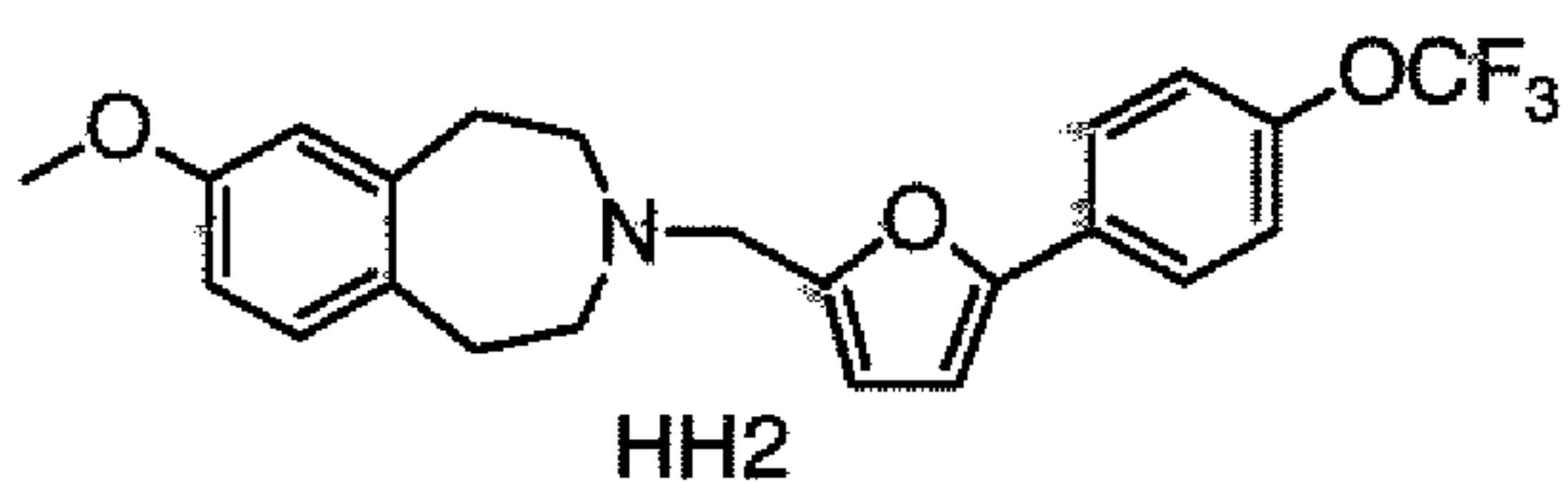
7-Methoxy-3-[5-(4-trifluoromethoxy-phenyl)-furan-2-ylmethyl]-2,3,4,5-tetrahydro-1H-benzo[d]azepine
