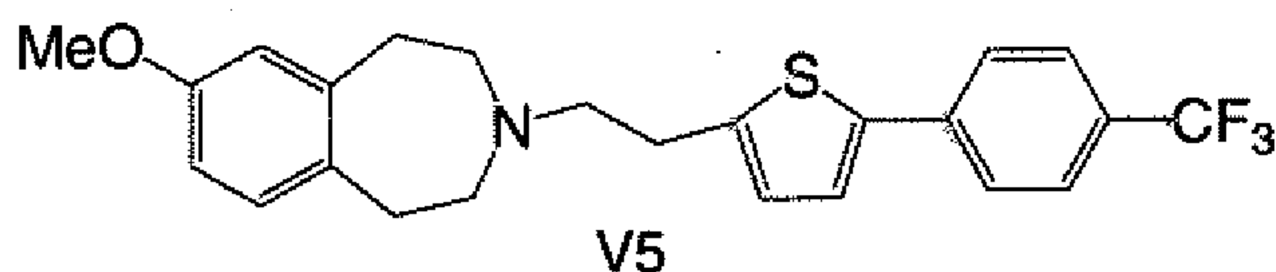
V5 7-Methoxy-3-{2-[5-(4-trifluoromethyl-phenyl)-thiophen-2-yl]-ethyl}-2,3,4,5-tetrahydro-1H-benzo[d]azepine
