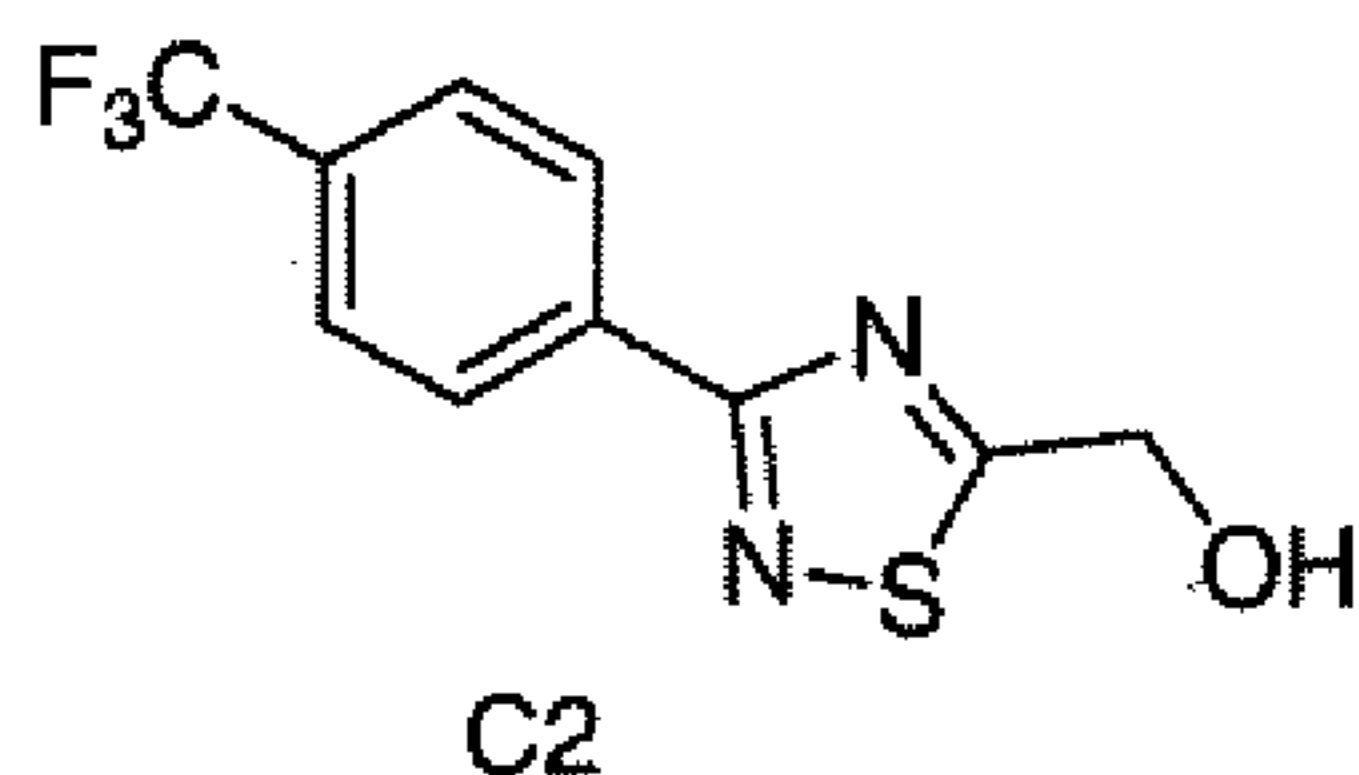
[3-(4-Trifluoromethyl-phenyl)-[1,2,4]thiadiazol-5-yl]-methanol
