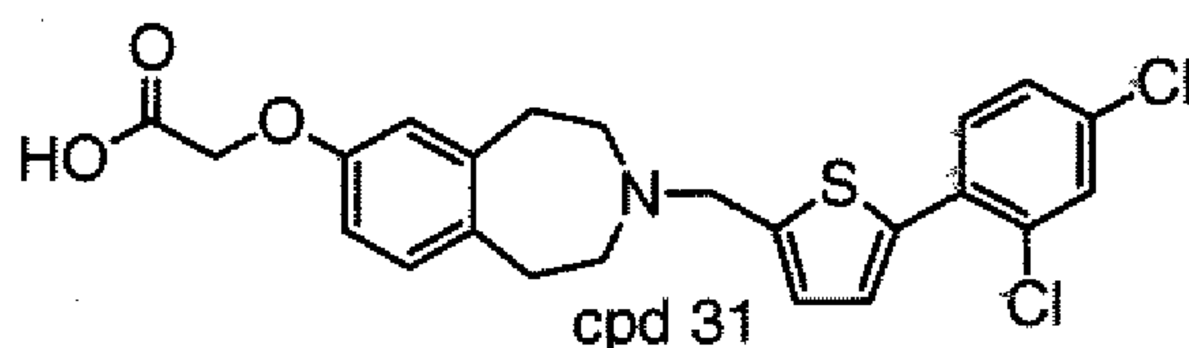
[3-[5-(2,4-Dichloro-phenyl)-thiophen-2-ylmethyl]-2,3,4,5-tetrahydro-1H-benzo[d]azepin-7-yloxy]-acetic acid
