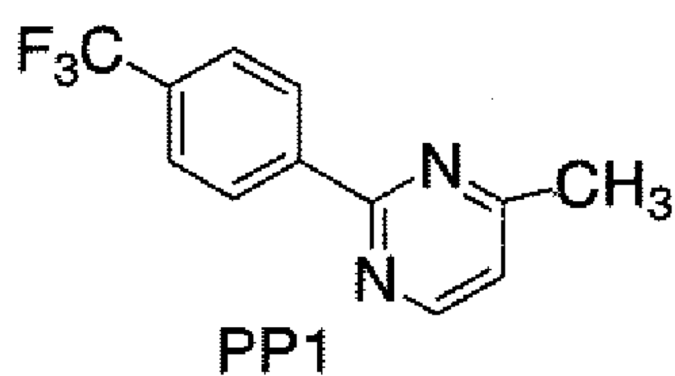
4-Methyl-2-(4-trifluoromethyl-phenyl)-pyrimidine
