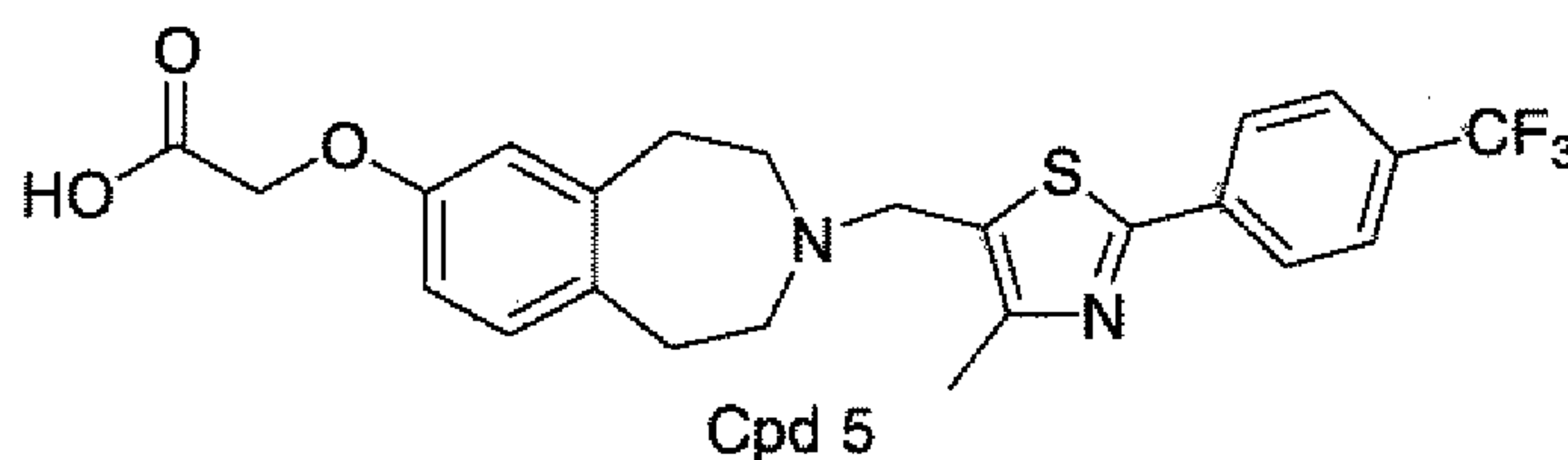
{3-[4-Methyl-2-(4-trifluoromethyl-phenyl)-thiazol-5-ylmethyl]-2,3,4,5-tetrahydro-1H-benzo[d]azepin-7-yloxy}-acetic acid
