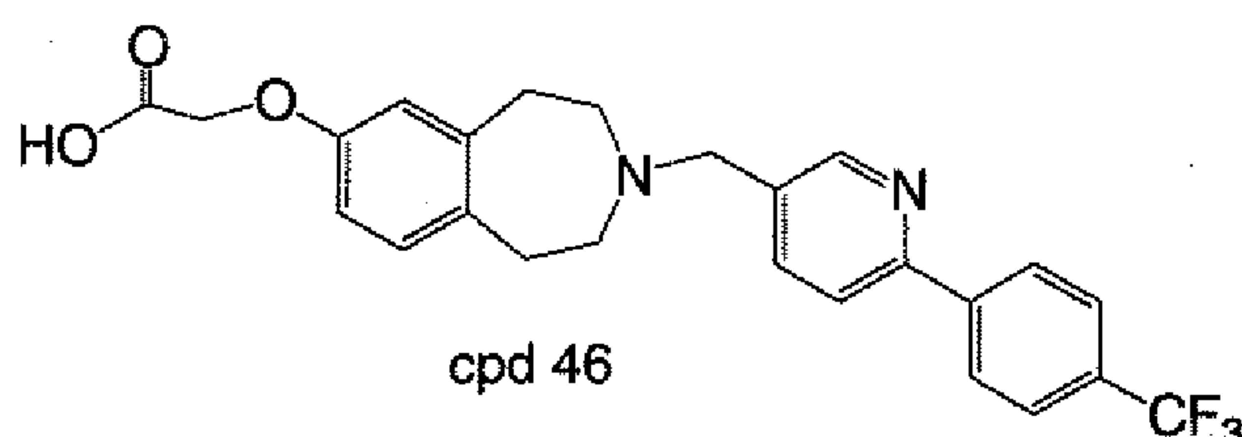
{3-[6-(4-Trifluoromethyl-phenyl)-pyridin-3-ylmethyl]-2,3,4,5-tetrahydro-1H-benzo[d]azepin-7-yloxy}-acetic acid
