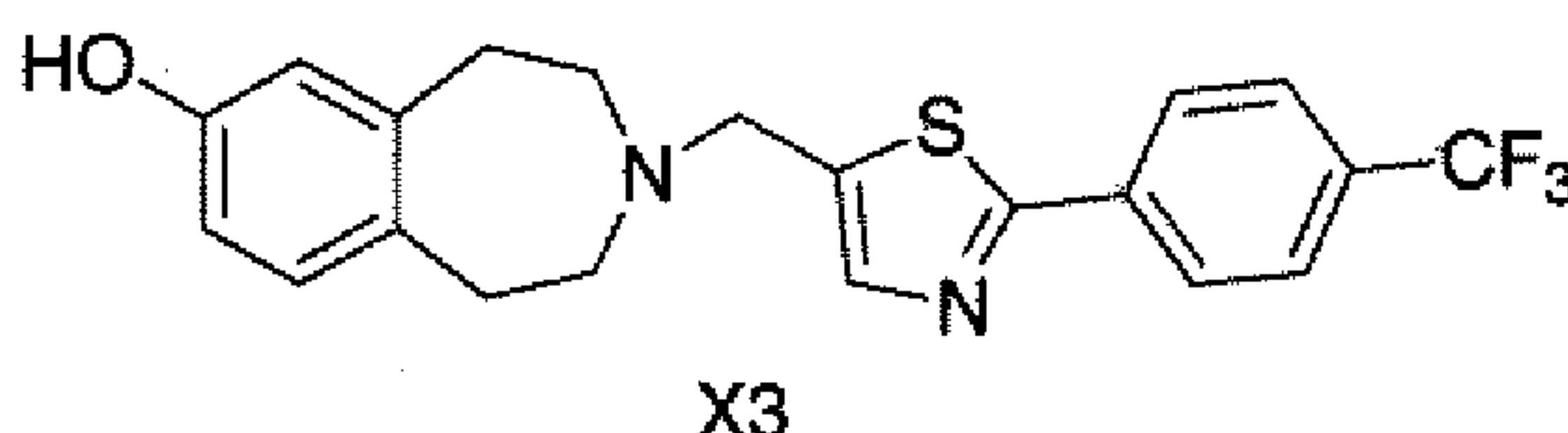
3-[2-(4-Trifluoromethyl-phenyl)-thiazol-5-ylmethyl]-2,3,4,5-tetrahydro-1H-benzo[d]azepin-7-ol
