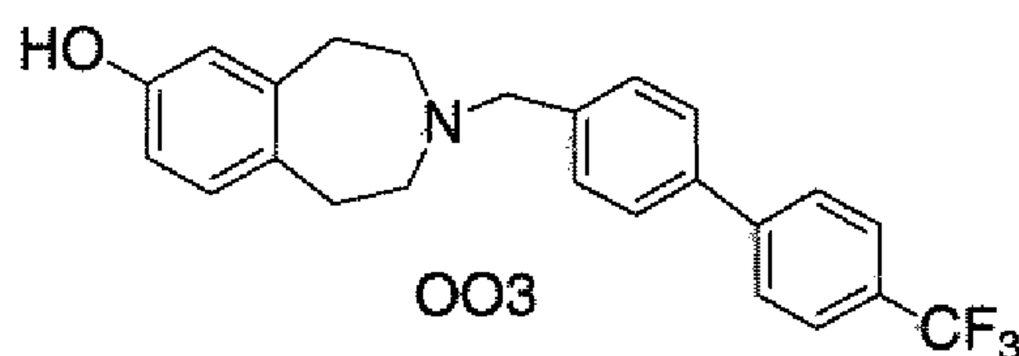
3-(4'-(Trifluoromethyl)-biphenyl-4-ylmethyl)-2,3,4,5-tetrahydro-1H-benzo[d]azepin-7-ol
