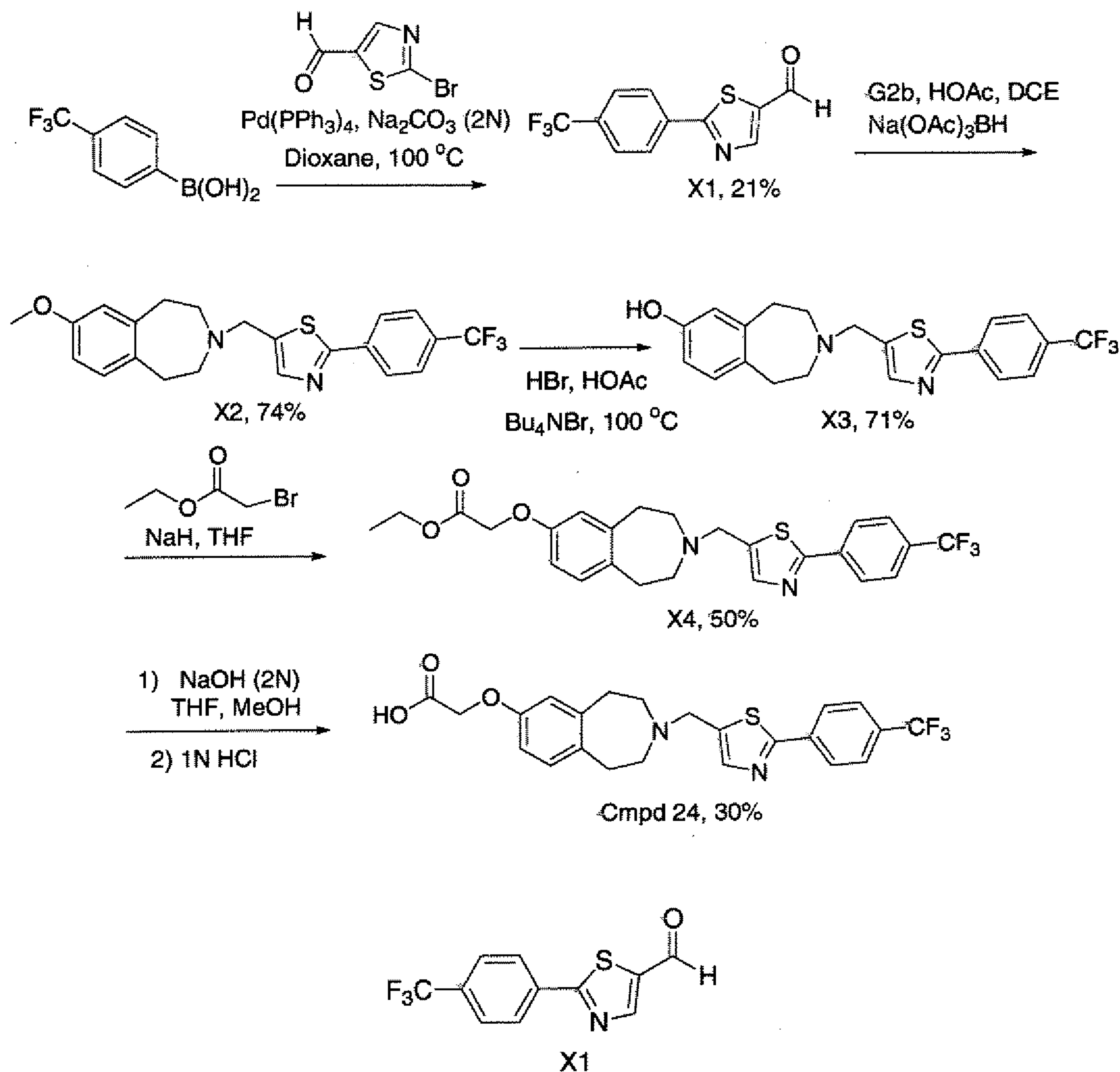
2-(4-Trifluoromethyl-phenyl)-thiazole-5-carbaldehyde
