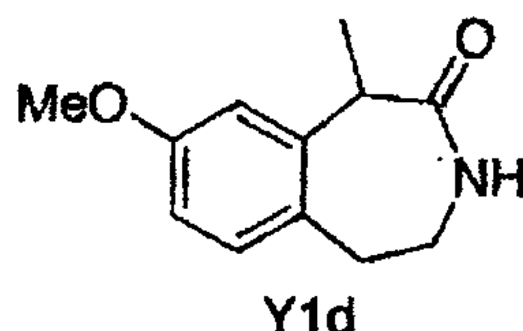
8-Methoxy-1-methyl-1,3,4,5-tetrahydro-benzo[d]azepin-2-one
