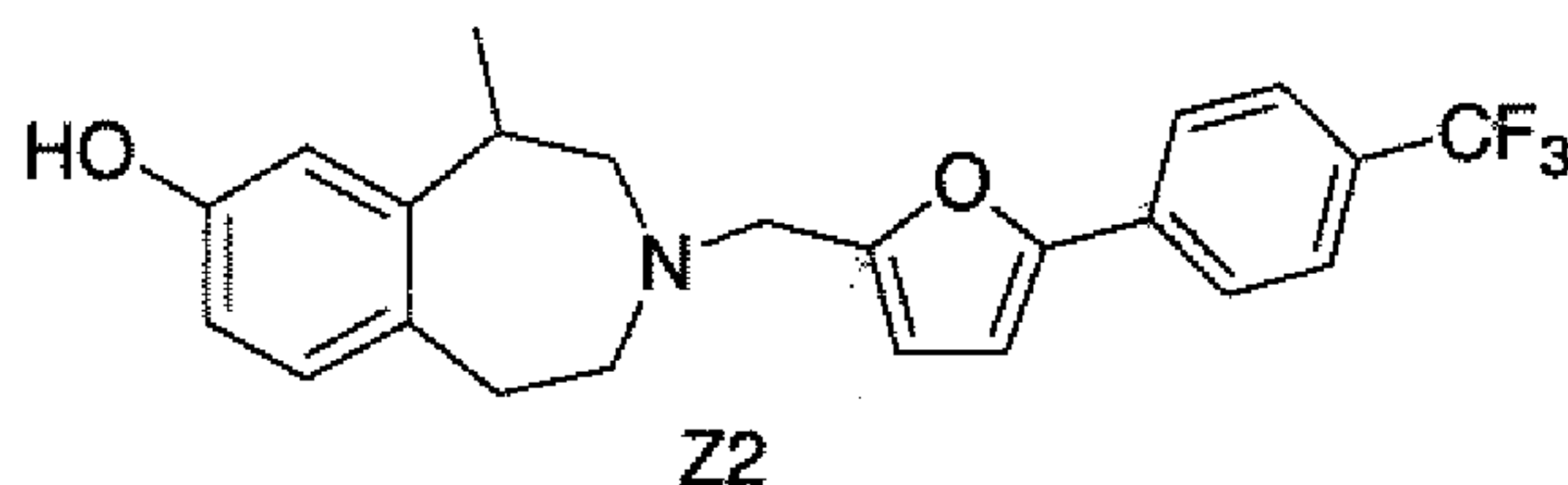
5-Methyl-3-[5-(4-trifluoromethyl-phenyl)-furan-2-ylmethyl]- 2,3,4,5-tetrahydro-1H-benzo[d]azepin-7-ol
