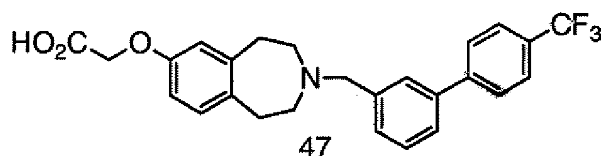
[3-(4'-Trifluoromethyl-biphenyl-3-ylmethyl)-2,3,4,5-tetrahydro-1H-benzo[d]azepin-7-yloxy]-acetic acid
