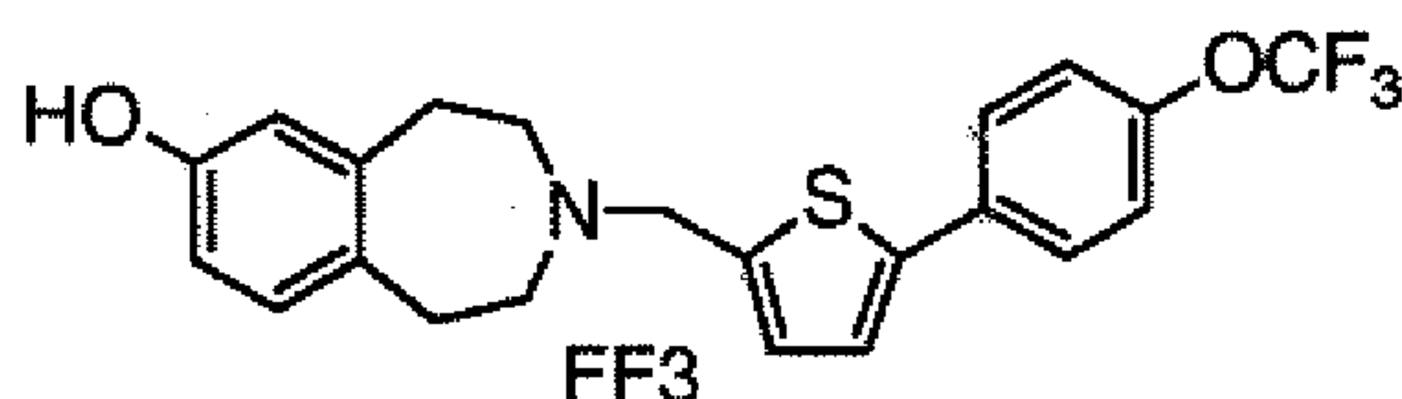
3-[5-(4-Trifluoromethoxy-phenyl)-thiophen-2-ylmethyl]-2,3,4,5-tetrahydro-1H-benzo[d]azepin-7-ol
