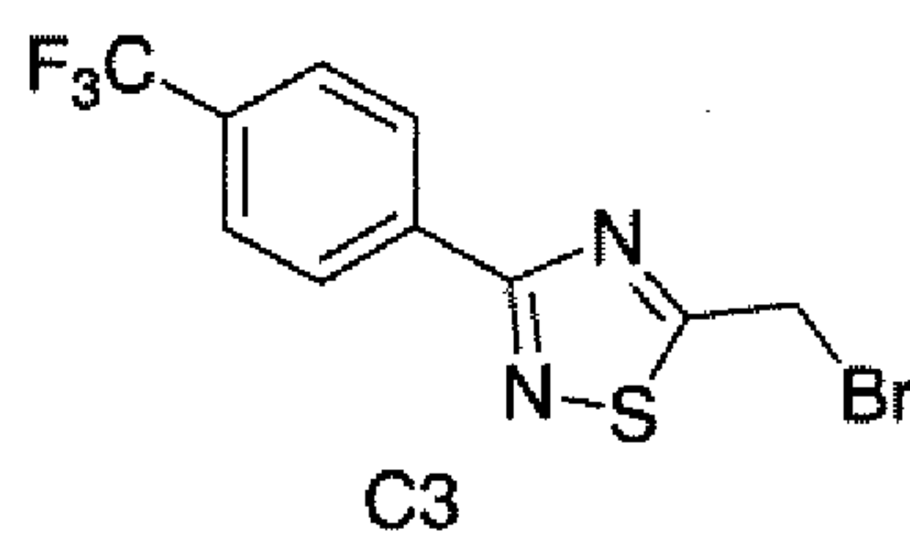
5-Bromomethyl-3-(4-trifluoromethyl-phenyl)-[1,2,4]thiadiazole
