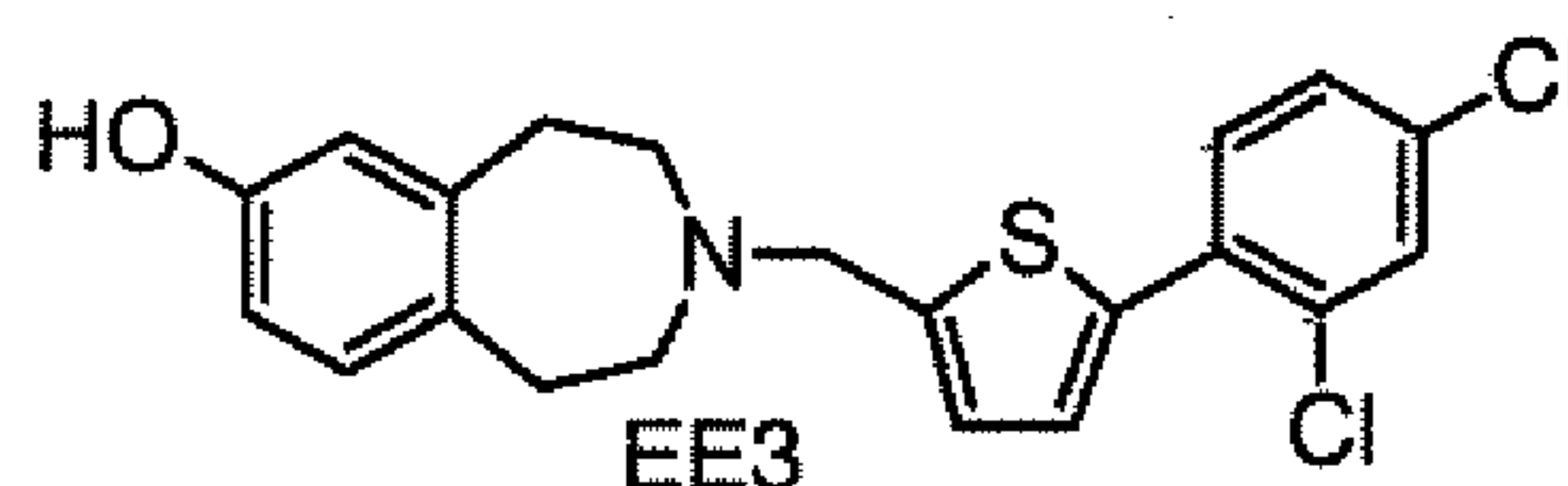
3-[5-(2,4-Dichloro-phenyl)-thiophen-2-ylmethyl]-2,3,4,5-tetrahydro-1H-benzo[d]azepin-7-ol
