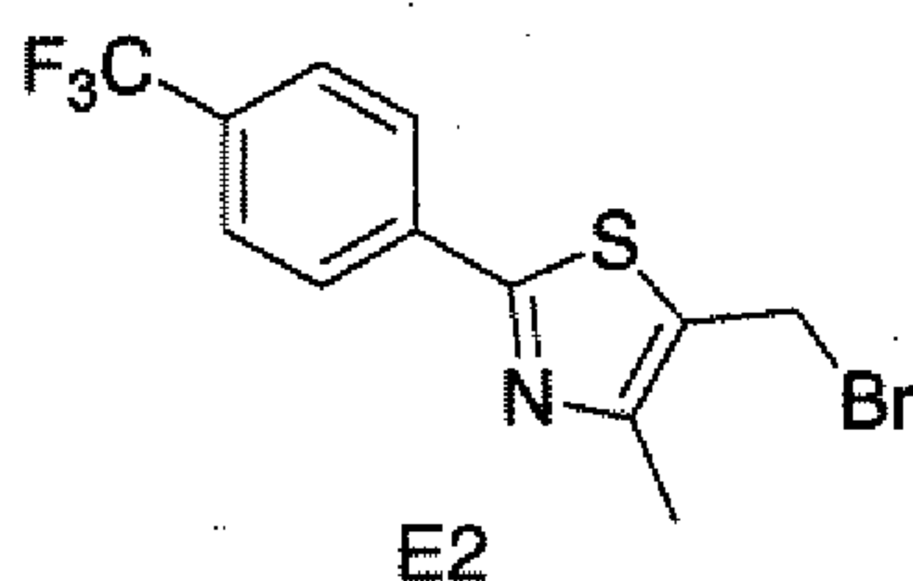
5-Bromomethyl-4-methyl-2-(4-trifluoromethyl-phenyl)-thiazole
