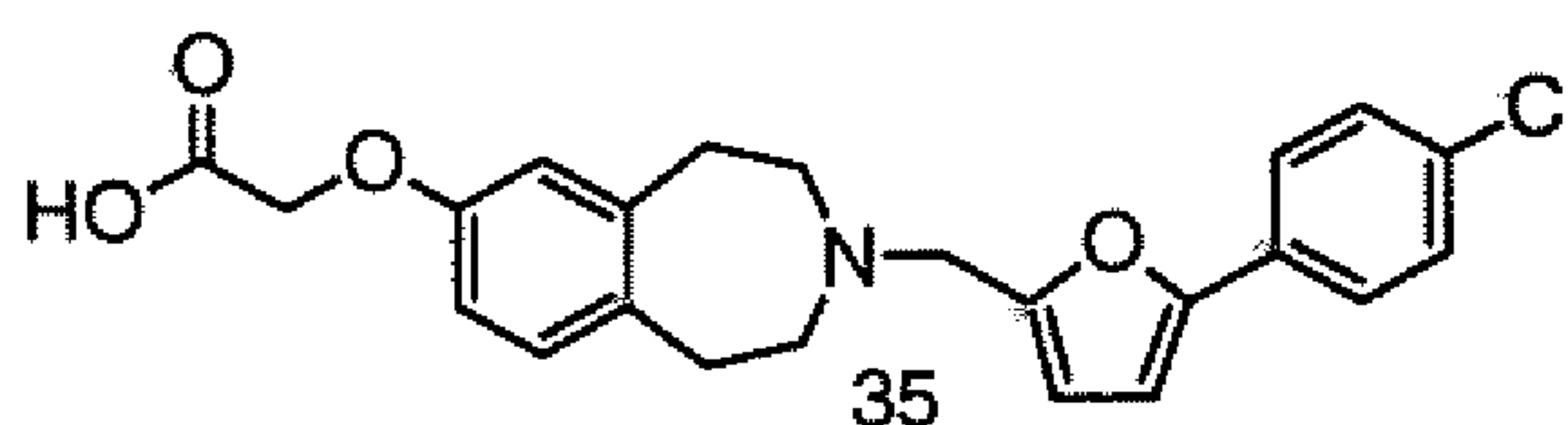
35 {3-[5-(4-Chloro-phenyl)-furan-2-ylmethyl]-2,3,4,5-tetrahydro-1H-benzo[d]azepin-7-yloxy}-acetic acid
