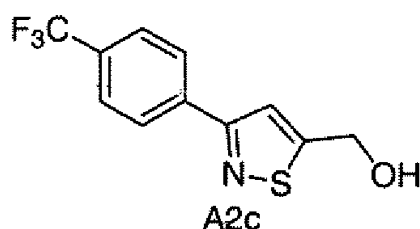
[3-(4-Trifluoromethyl-phenyl)-isothiazol-5-yl]-methanol
