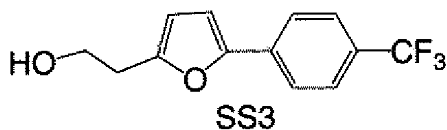
2-[5-(4-Trifluoromethyl-phenyl)-furan-2-yl]-ethanol
