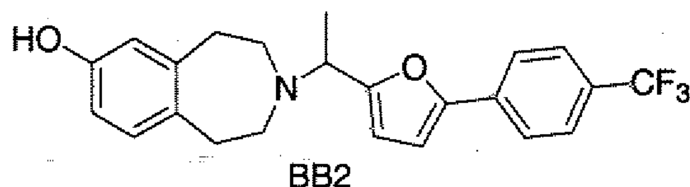
3-{1-[5-(4-Trifluoromethyl-phenyl)-furan-2-yl]-ethyl}-2,3,4,5-tetrahydro-1H-benzo[d]azepin-7-ol
