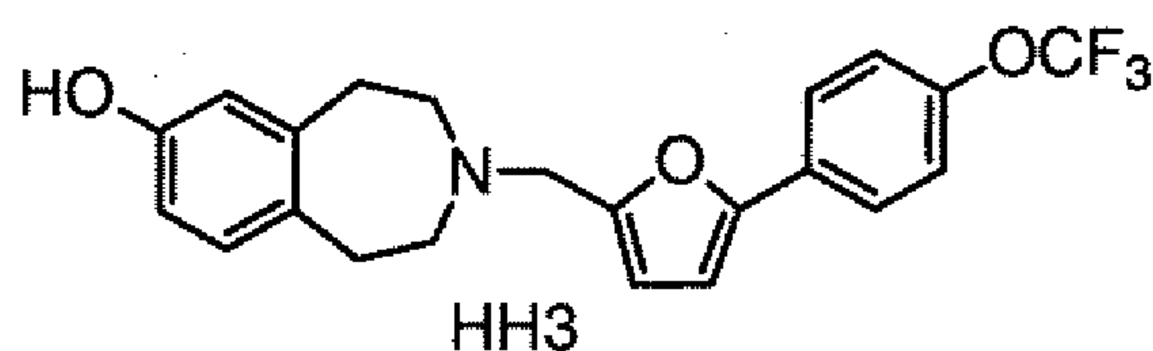
3-[5-(4-Trifluoromethoxy-phenyl)-furan-2-ylmethyl]-2,3,4,5-tetrahydro-1H-benzo[d]azepin-7-ol
