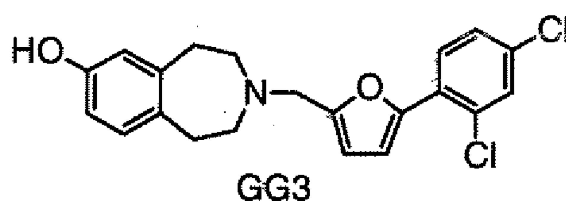
GG3 3-[5-(2,4-Dichloro-phenyl)-furan-2-ylmethyl]-2,3,4,5-tetrahydro-1H-benzo[d]azepin-7-ol
