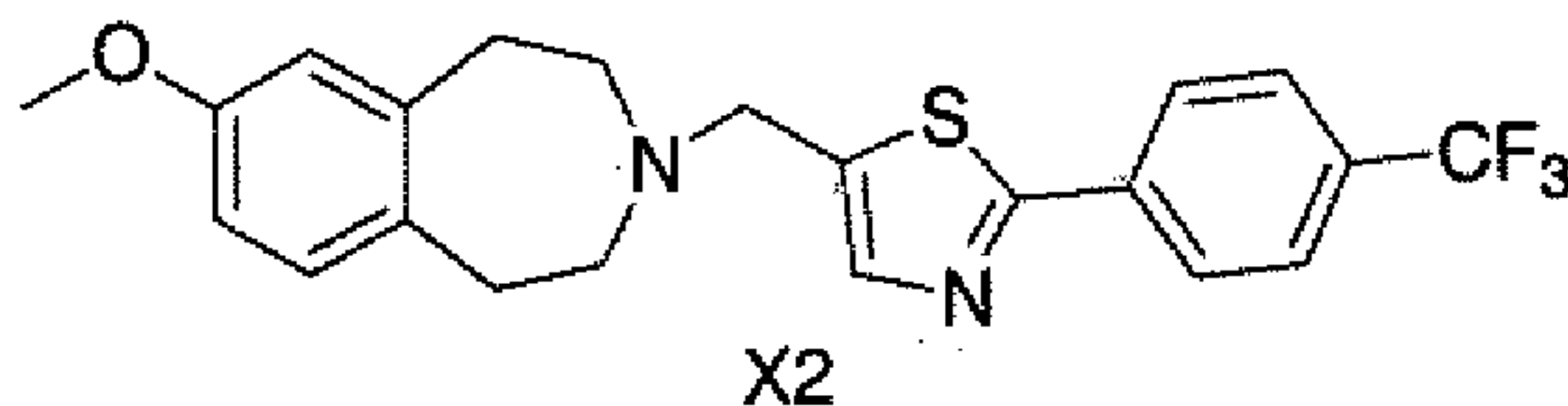
7-Methoxy-3-[2-(4-trifluoromethyl-phenyl)-thiazol-5-ylmethyl]-2,3,4,5-tetrahydro-1H-benzo[d]azepine
