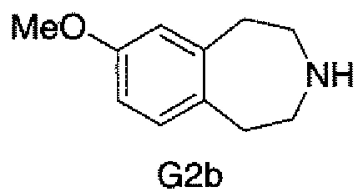
7-Methoxy-2,3,4,5-tetrahydro-1H-benzo[d]azepine
