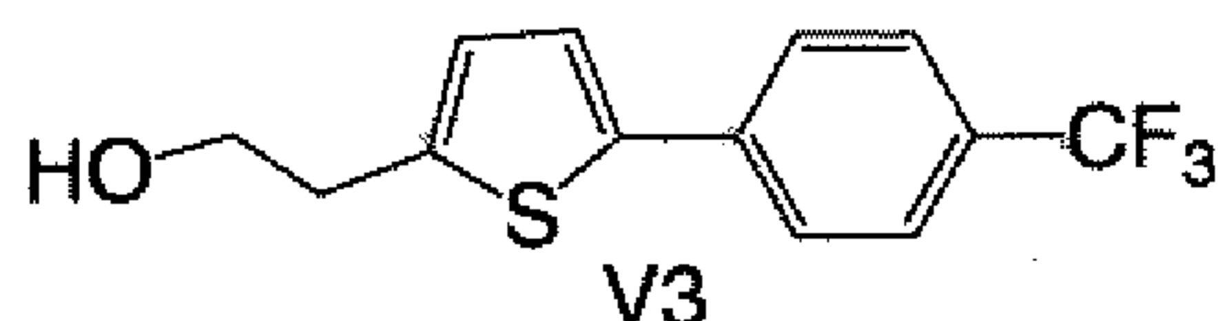
2-[5-(4-Trifluoromethyl-phenyl)-thiophen-2-yl]-ethanol
