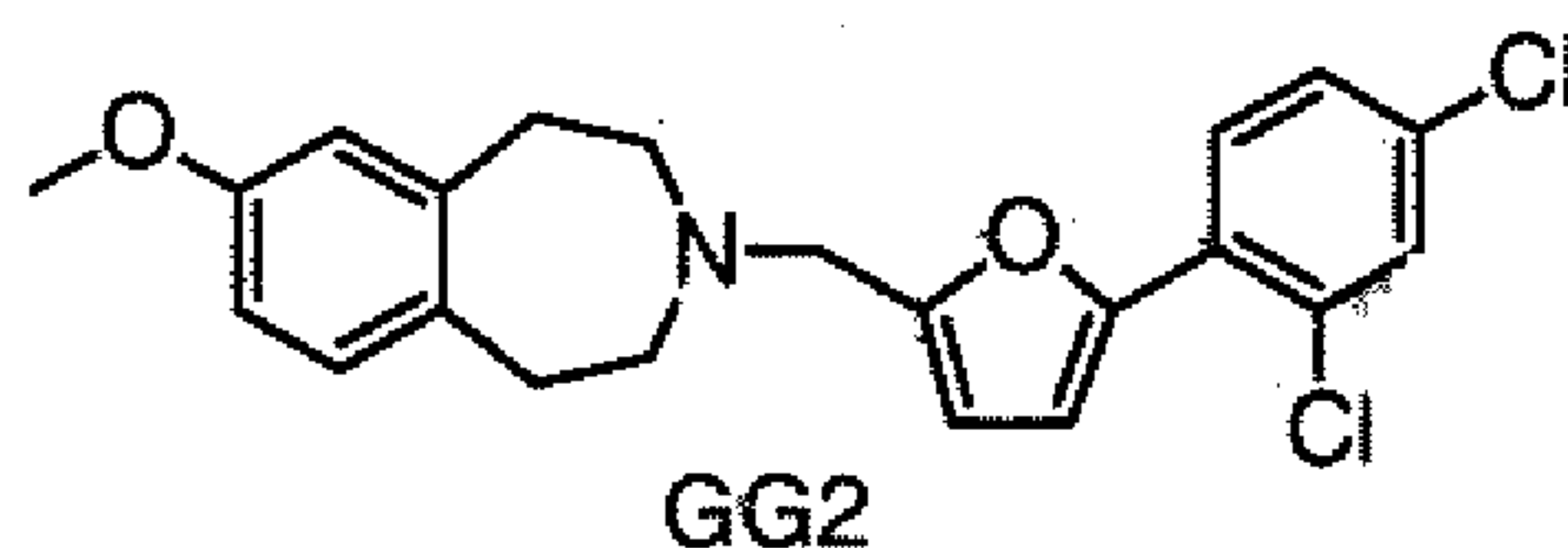
GG2 3-[5-(2,4-Dichloro-phenyl)-furan-2-ylmethyl]-7-methoxy-2,3,4,5-tetrahydro-1H-benzo[d]azepine
