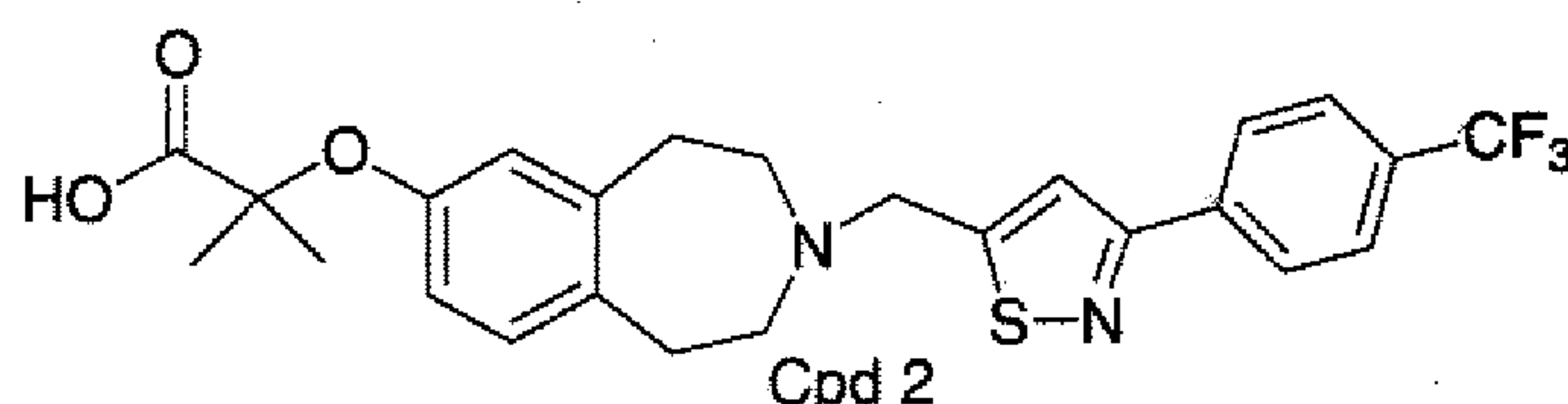
2-Methyl-2-{3-[3-(4-trifluoromethyl-phenyl)-isothiazol-5-ylmethyl]-2,3,4,5-tetrahydro-1H-benzo[d]azepin-7-yloxy}-propionic acid
