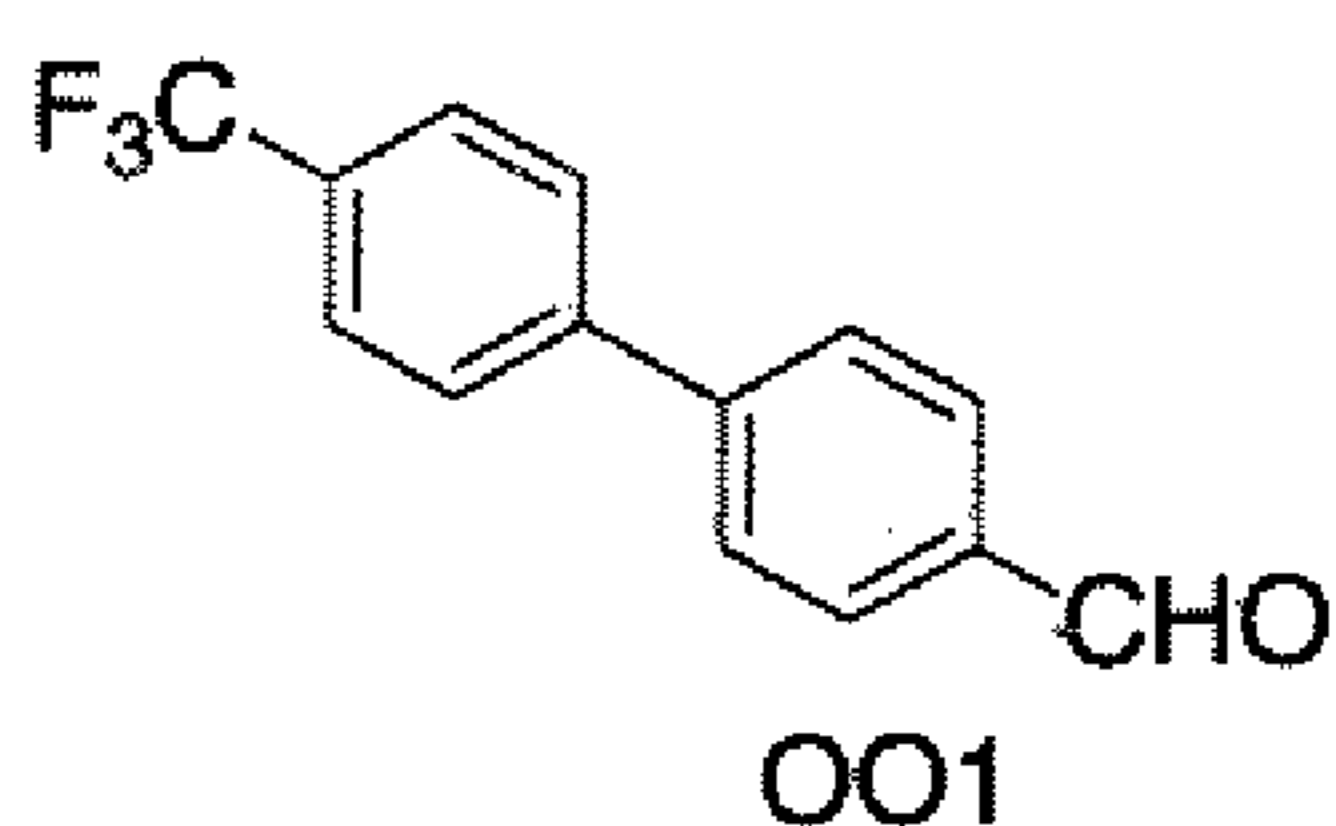
4'-(Trifluoromethyl)-biphenyl-4-carbaldehyde
