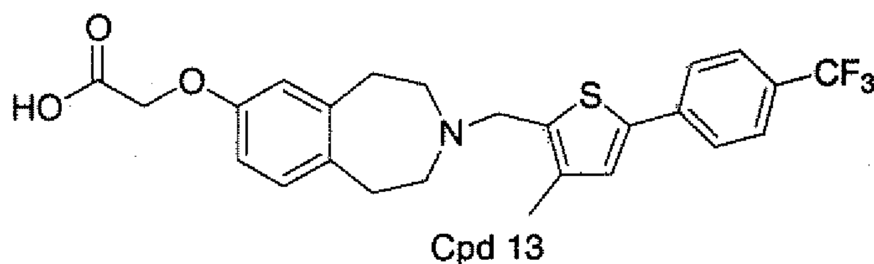
{3-[3-Methyl-5-(4-trifluoromethyl-phenyl)-thiophen-2-ylmethyl]-2,3,4,5-tetrahydro-1H-benzo[d]azepin-7-yloxy}-acetic acid
