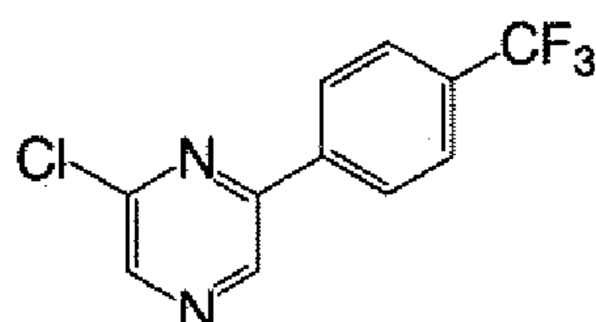
2-Chloro-6-(4-trifluoromethyl-phenyl)-pyrazine
