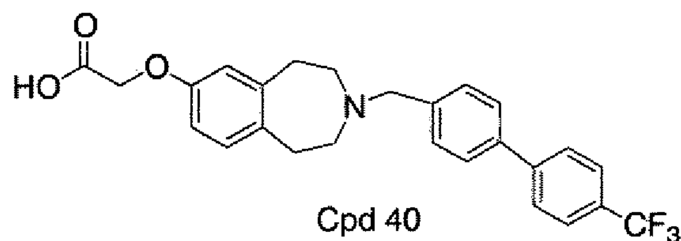
[3-(4'-Trifluoromethyl-biphenyl-4-ylmethyl)-2,3,4,5-tetrahydro-1H-benzo[d]azepin-7-yloxy]-acetic acid
