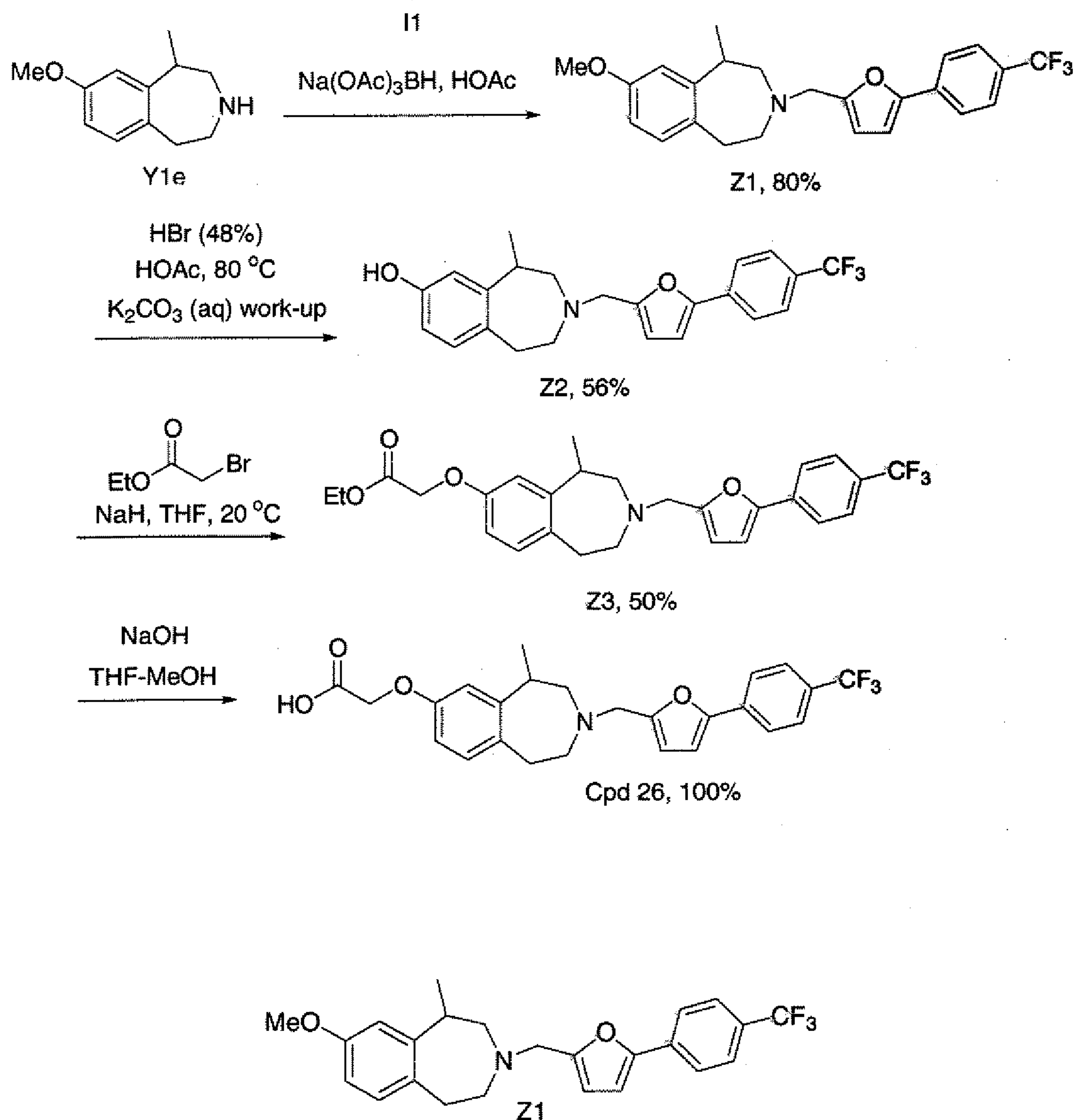
8-Methoxy-1-methyl-3-[5-(4-trifluoromethyl-phenyl)-furan-2-ylmethyl]- 2,3,4,5-tetrahydro-1H-benzo[d]azepine
