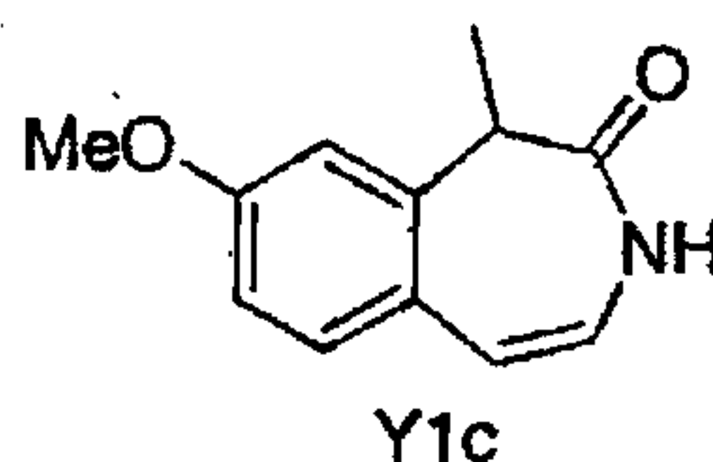
8-Methoxy-1-methyl-1,3-dihydro-benzo[d]azepin-2-one
