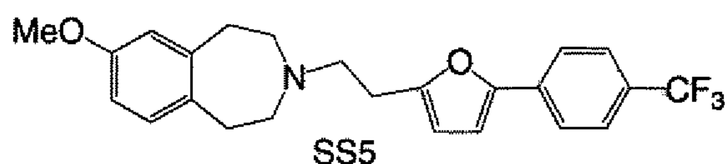
7-Methoxy-3-{2-[5-(4-trifluoromethyl-phenyl)-furan-2-yl]-ethyl}-2,3,4,5-tetrahydro-1H-benzo[d]azepine
