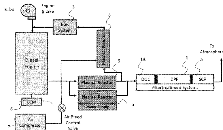
Calibrated Non-Thermal Plasma System with Multiple Reactors
