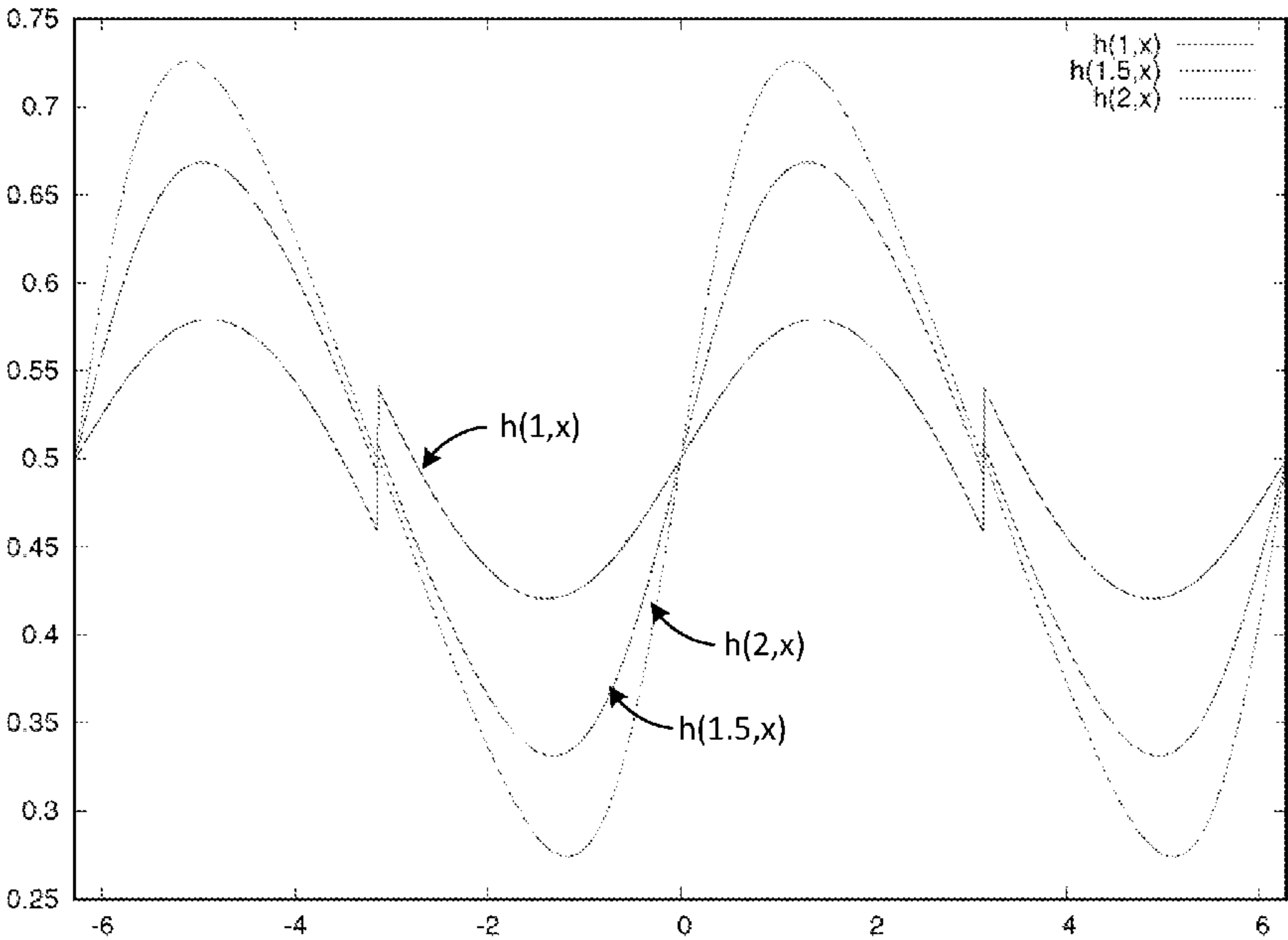
FIG. 2 Asymptotic approximation of the sigmoid via Theorem 1
