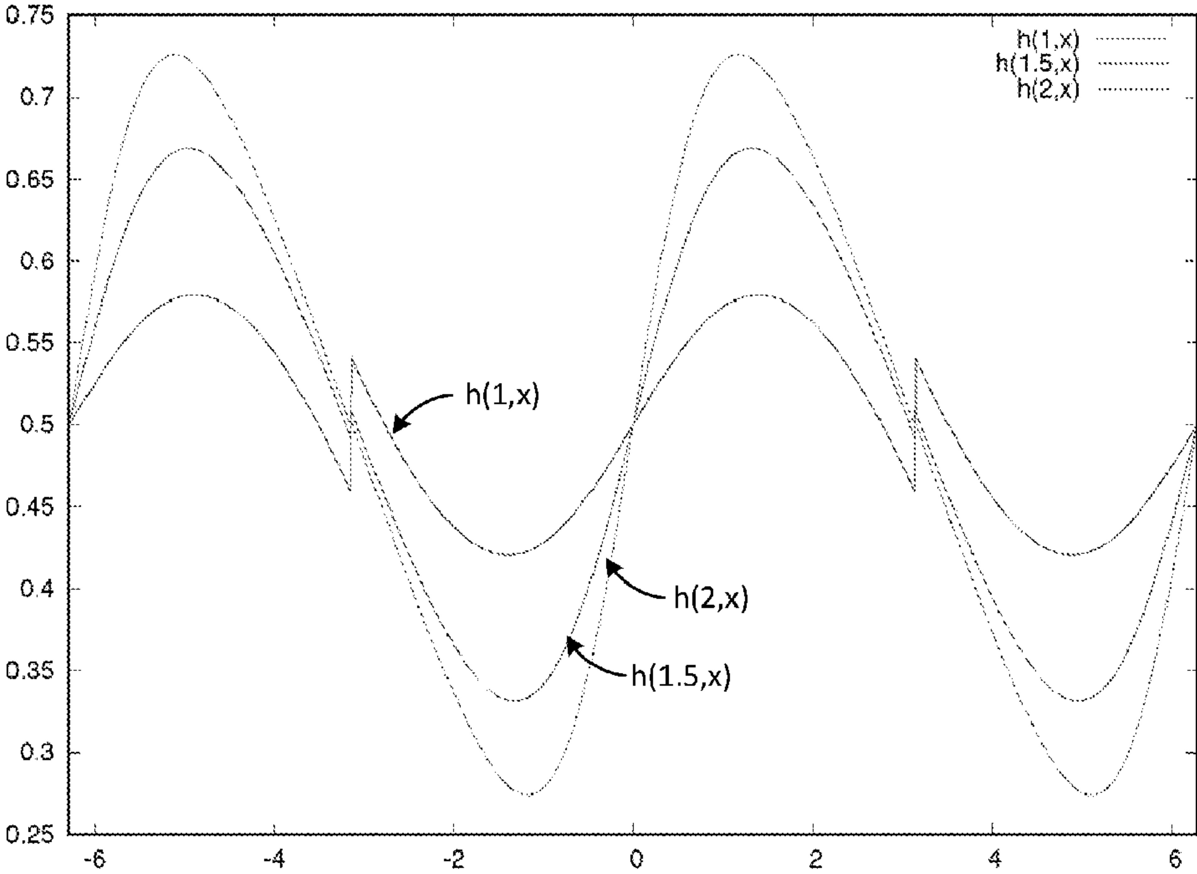
FIG. 2 Asymptotic approximation of the sigmoid via Theorem 1
