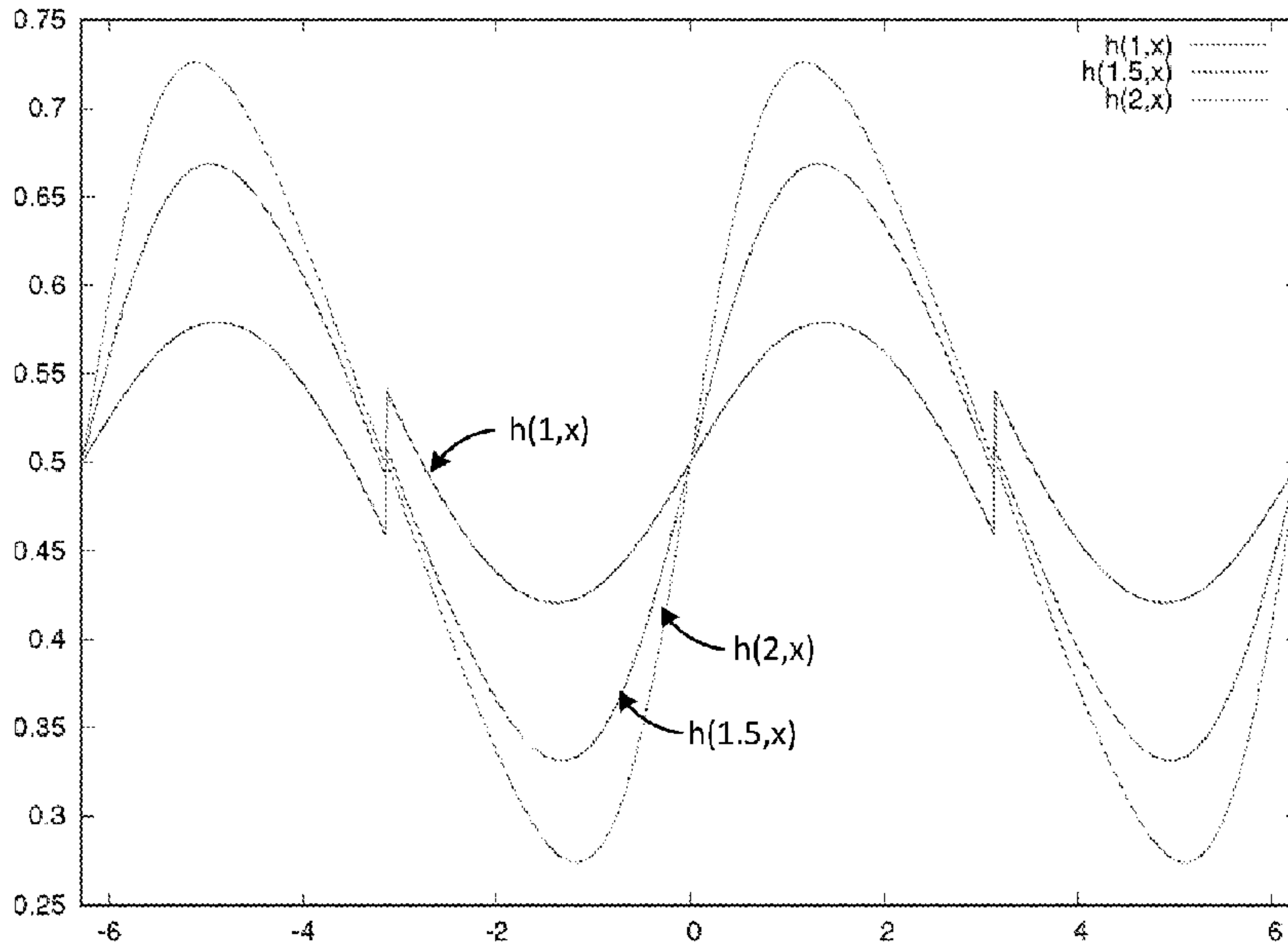
FIG. 2 Asymptotic approximation of the sigmoid via Theorem 1
