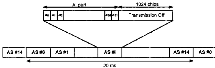
Figure 84: Structure of the AICH
