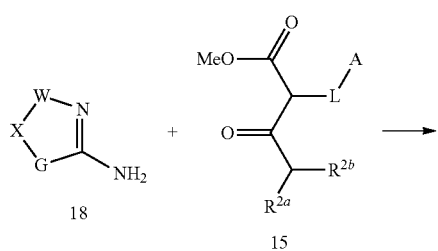
Scheme 5
