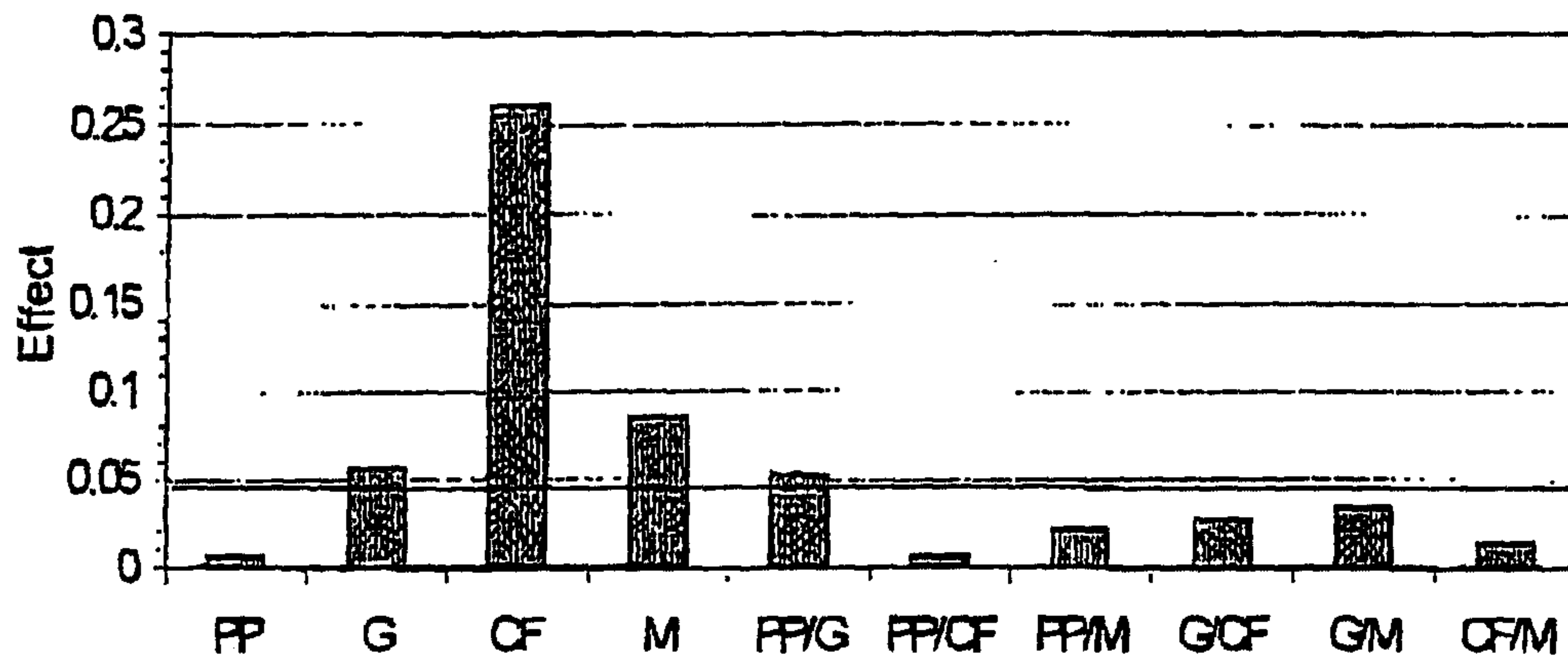
Pareto Chart for Coefficient of Friction
