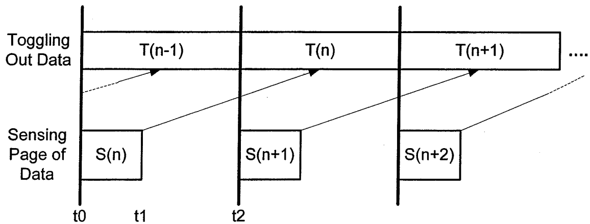
Conventional Read Caching
