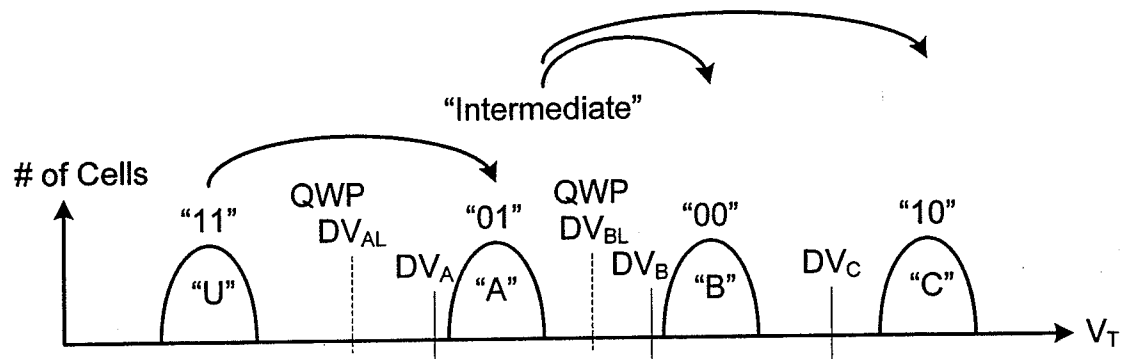
Upper Page Programming (LM Gray Code)
