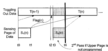
Read Caching with LM Coding (special case of reading lower logical page when upper page is not yet programmed)
