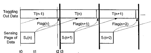
Read Caching with LM Coding
