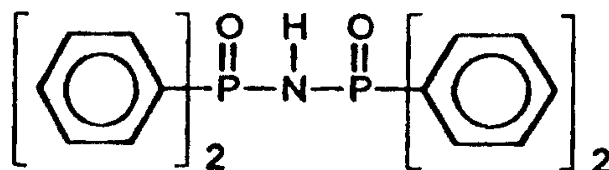
Imidotetraphenyldiphosphinic acid
