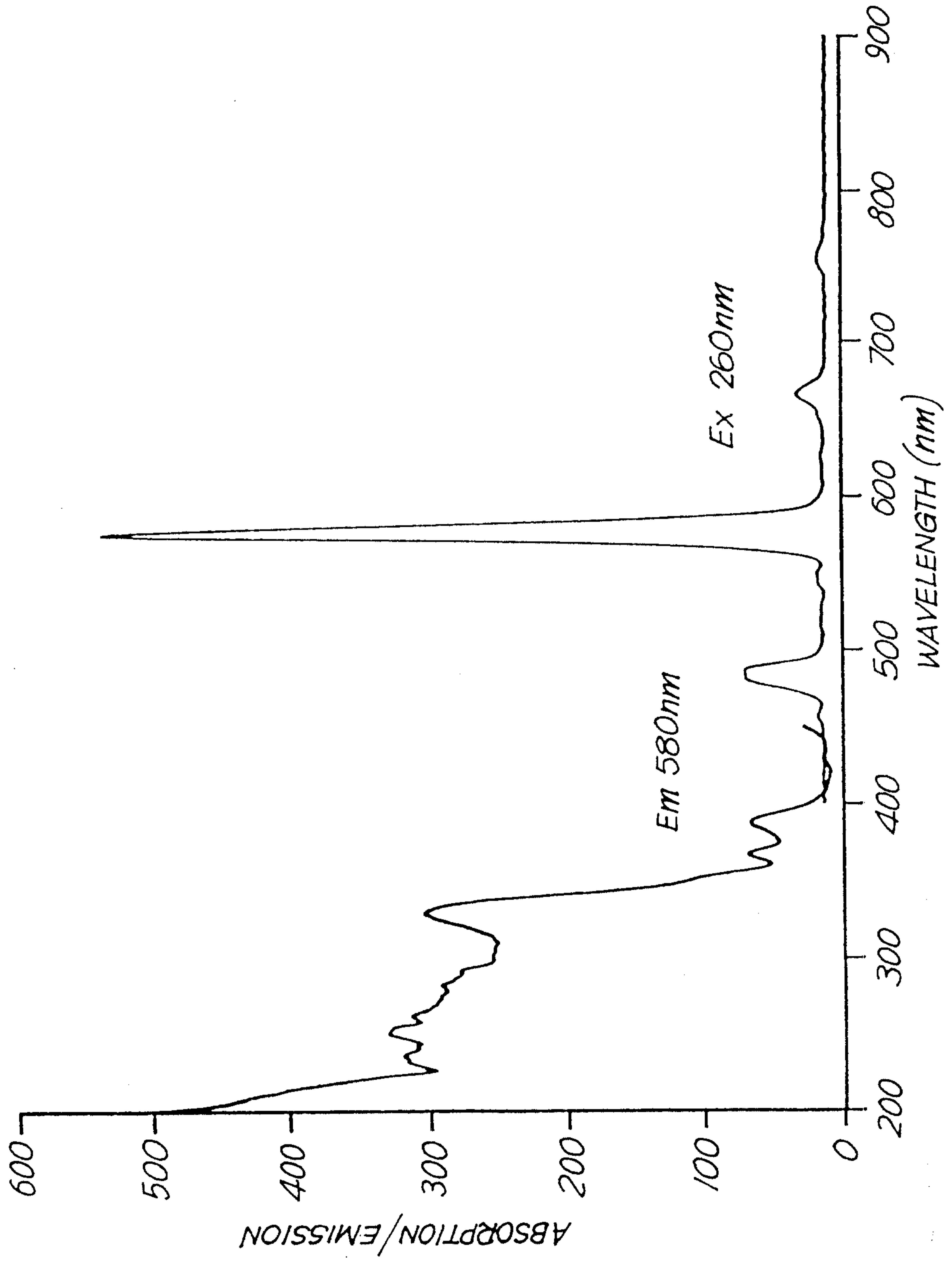
Fig.11 Excitation/Emission Spectra of Tris(2,2,6,6-tetramethyl-3,5-heptanedionato)dysprosium(III) Diphenylphosphonimido triphenylphosphorane
