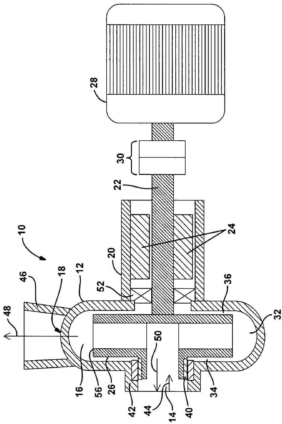
FIG. 1 Prior Art
