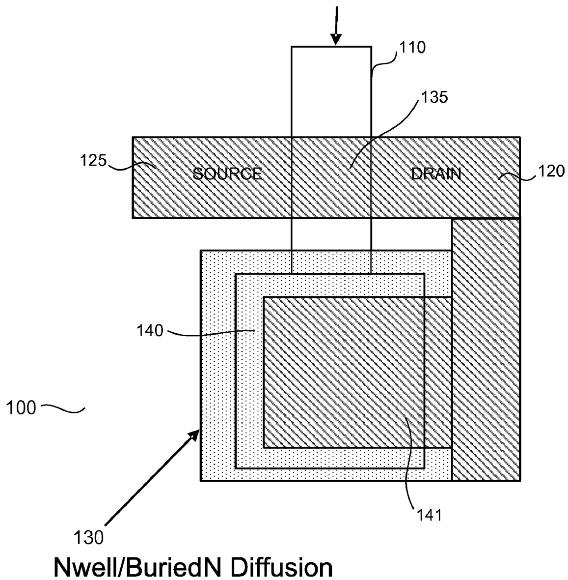
FIG. 1 Floating Gate
