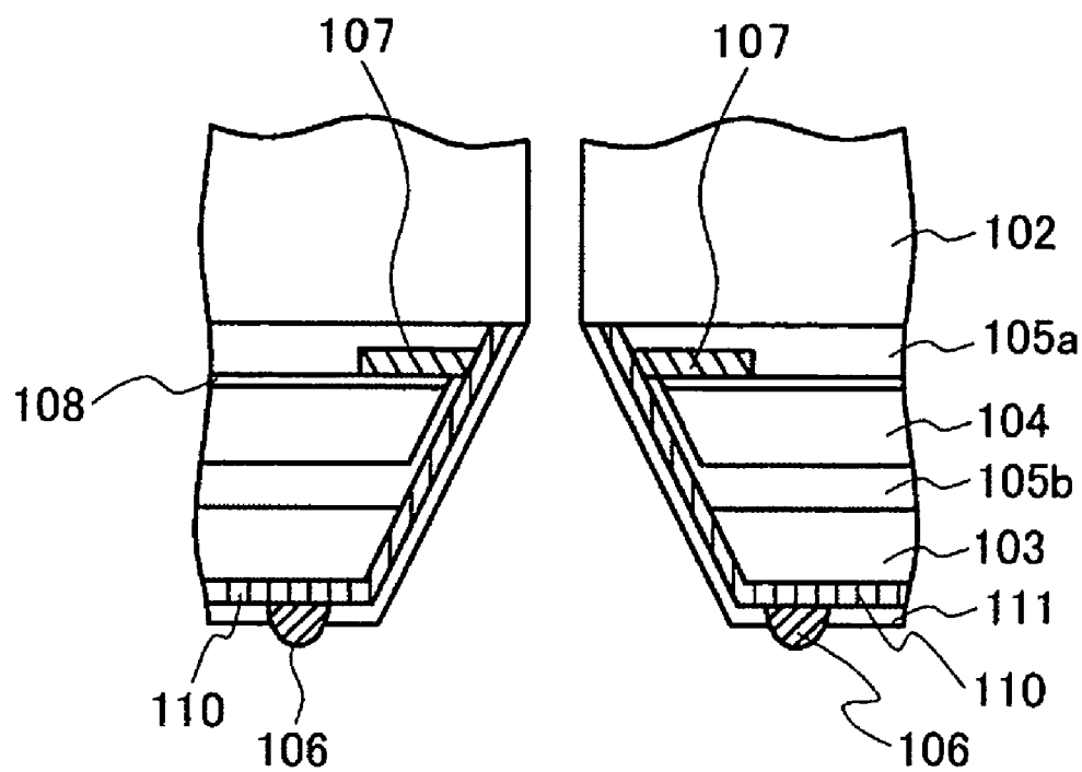
FIG. 10 PRIOR ART
