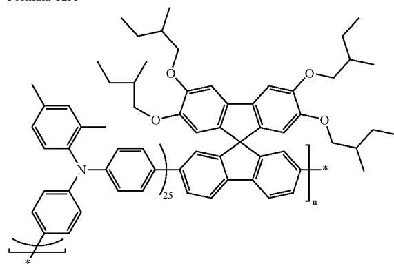
M_n = 17900 Formula 12B
