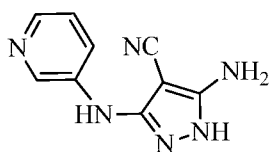
5-amino-3-(pyridin-3-ylamino)-1 H -pyrazole-4-carbonitrile
