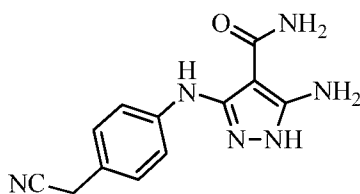
5-amino-3-((4-(cyanomethyl)phenyl)amino)-1 H -pyrazole-4-carboxamide
