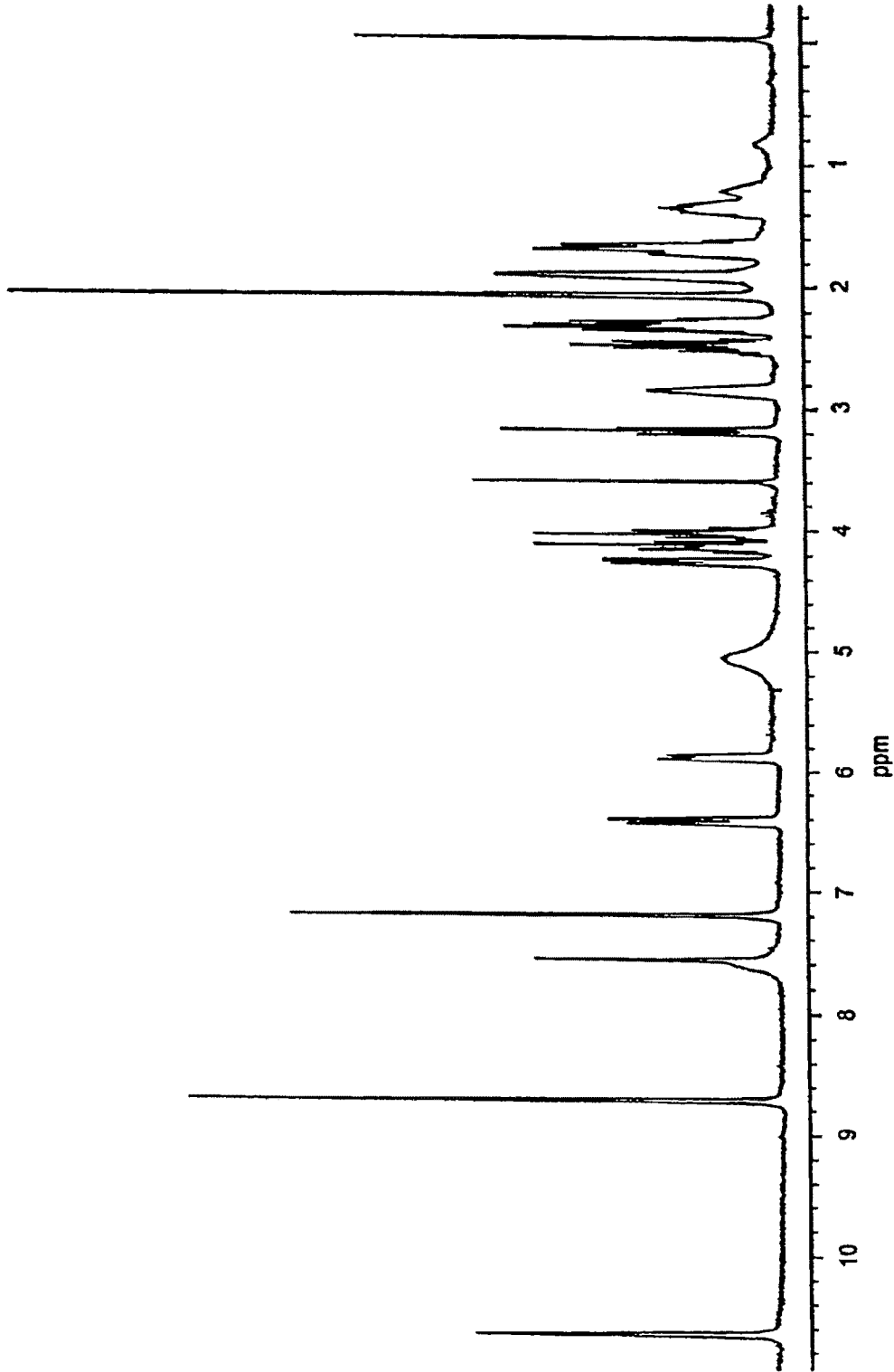
1 H-NMR of salinosporamide A (1), 300 MHz, d 5 -pyridine
