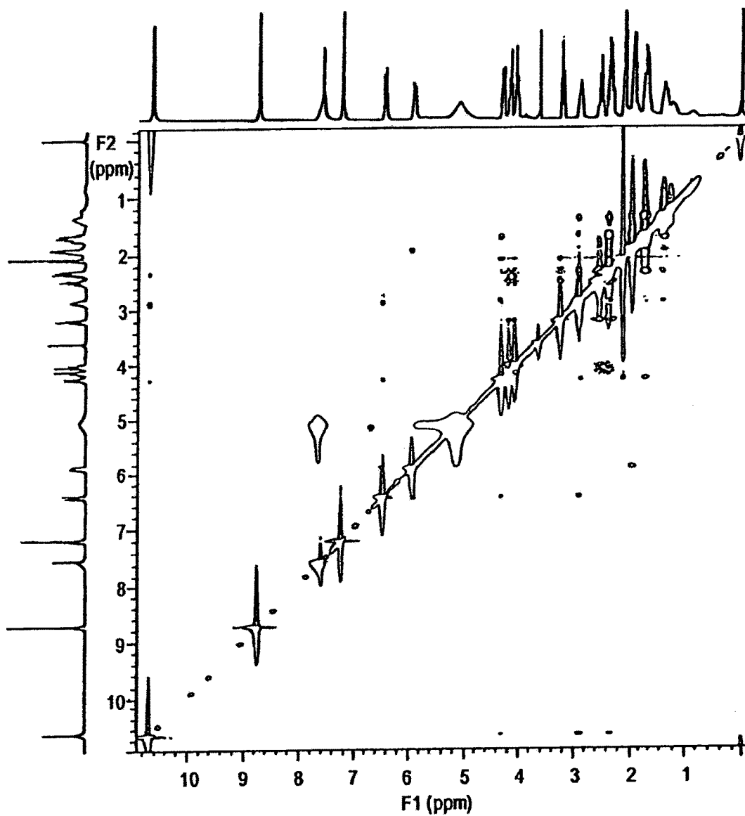
NOESY of salinosporamide A (1), 300 MHz, d 5 -pyridine
