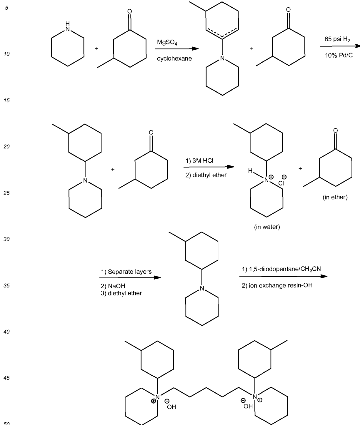
Scheme 1
