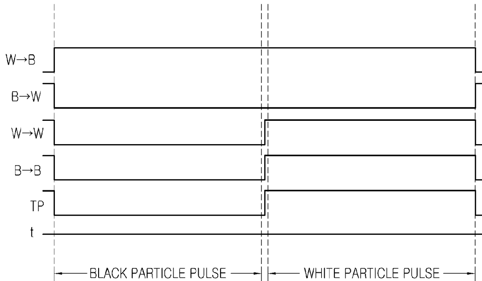
FIG.5 (PRIOR ART)
