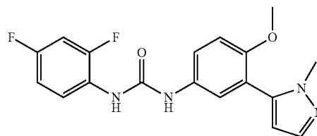
1-(2,4-difluorophenyl)-3-(4-methoxy-3-(1-methyl-1H-pyrazol-5-yl)phenyl)urea
