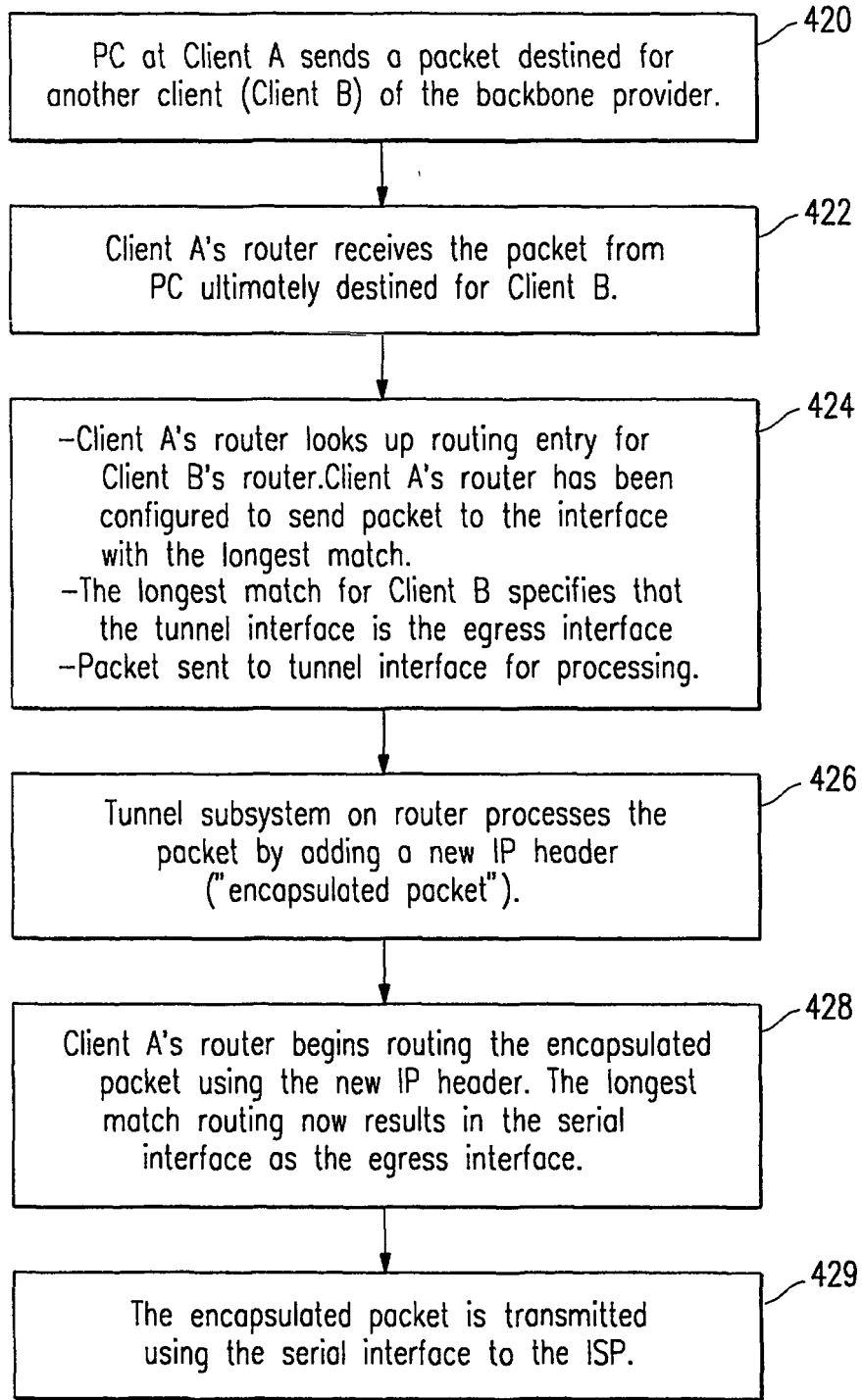
Routing on First Client Router
