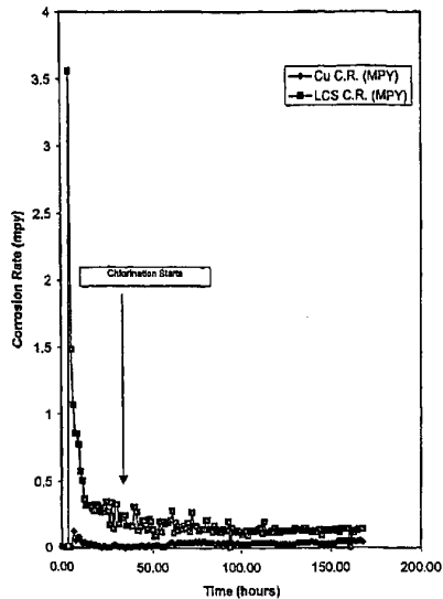
Low carbon steel and copper corrosion rate for the treatment containing 3 ppm example 19 (5-benzylbenzotriazole)
