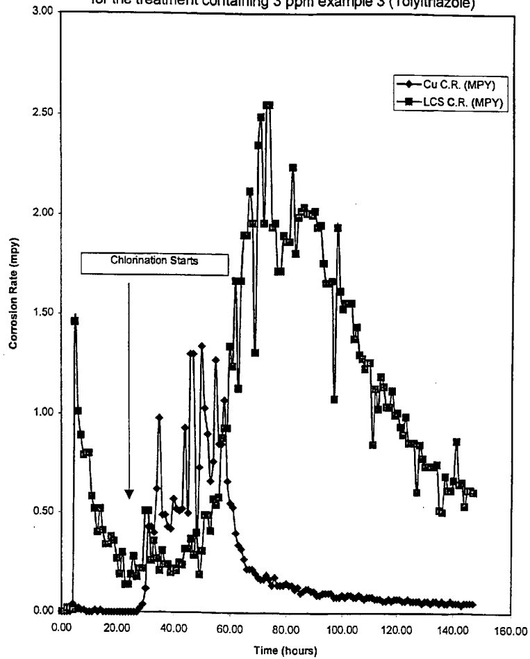
Figure 1. Low carbon steel and copper corrosion rate for the treatment containing 3 ppm example 3 (Tolyltriazole)
