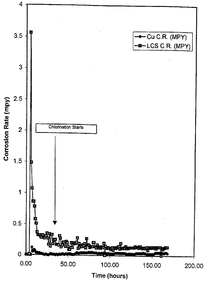
Figure 3. Low carbon steel and copper corrosion rate for the treatment containing 3 ppm example 19 (5-benzylbenzotriazole)
