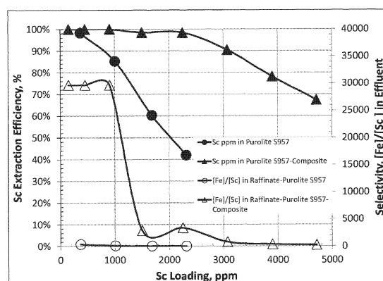
Figure 1. Column Process results of using Purolite S957 and Purolite S957-DEHPA for extracting rare earth metals from acid-leaching solution that contain a large amount of ferric ions.
