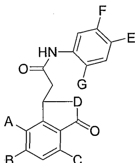
FORMULA II(H)
