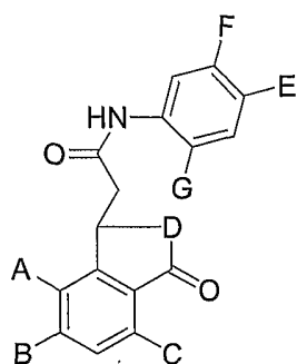
FORMULA II(H)
