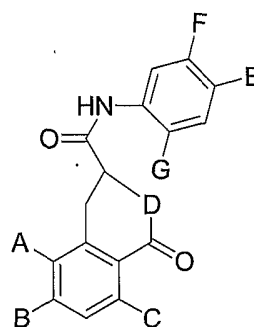
FORMULA II(I)
