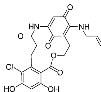
ALLYL AMINE
