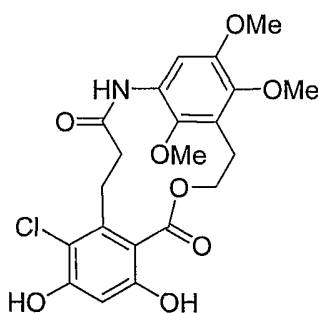
1,4-METHYL ETHER
