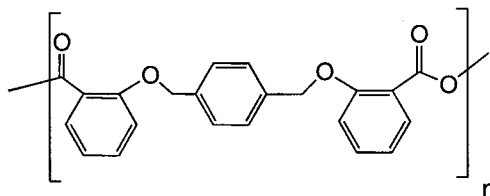
xylyl-based polymer
