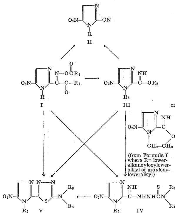
FLOW DIAGRAM
