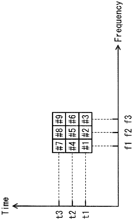
FIG. 72B Modulated signal z2
