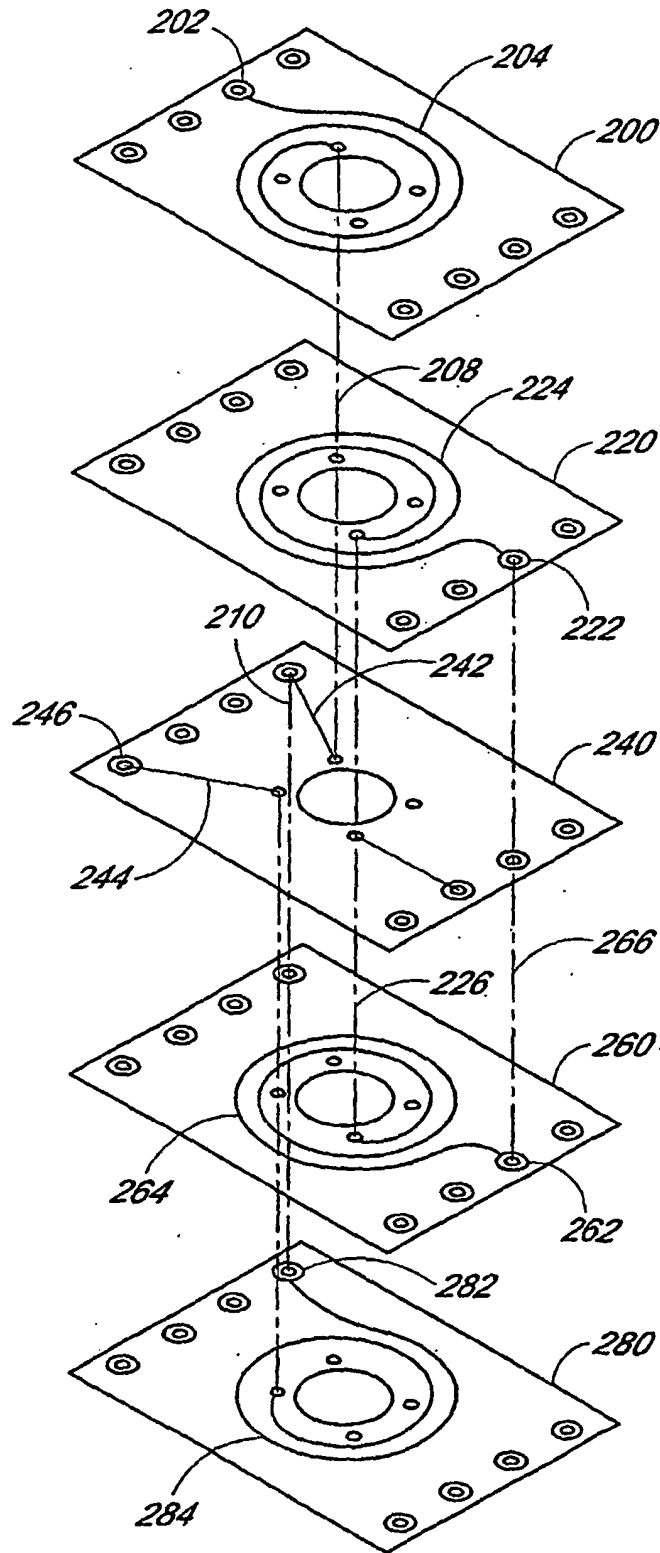
FIG. 2 (PRIOR ART)
