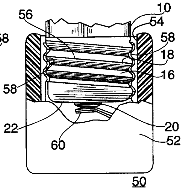
FIG. 6 PRIOR ART
