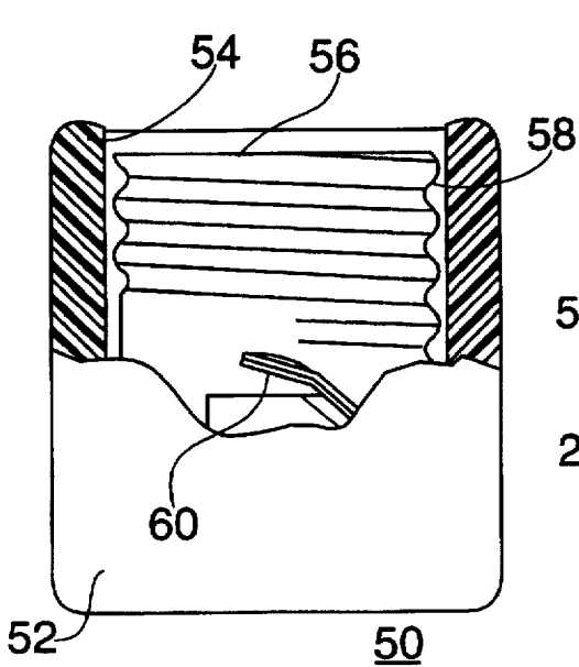
FIG. 5 PRIOR ART
