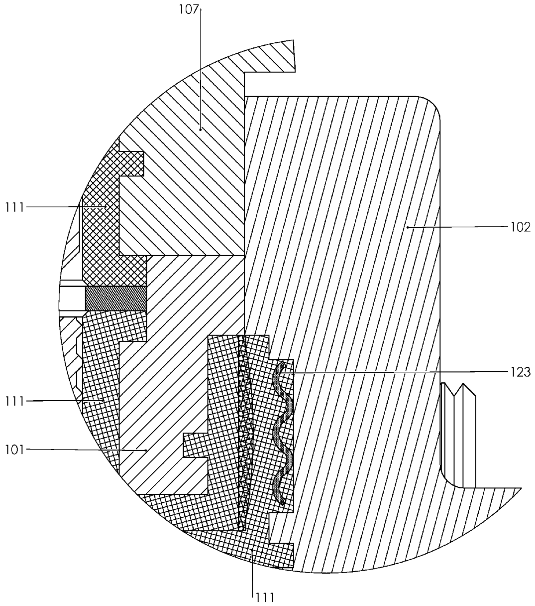
DETAIL III FIG. 5
