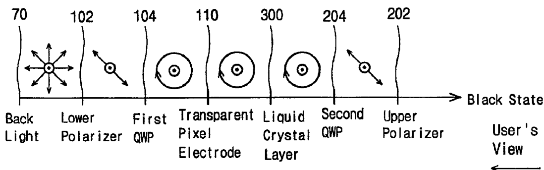
(related art) FIG. 4B
