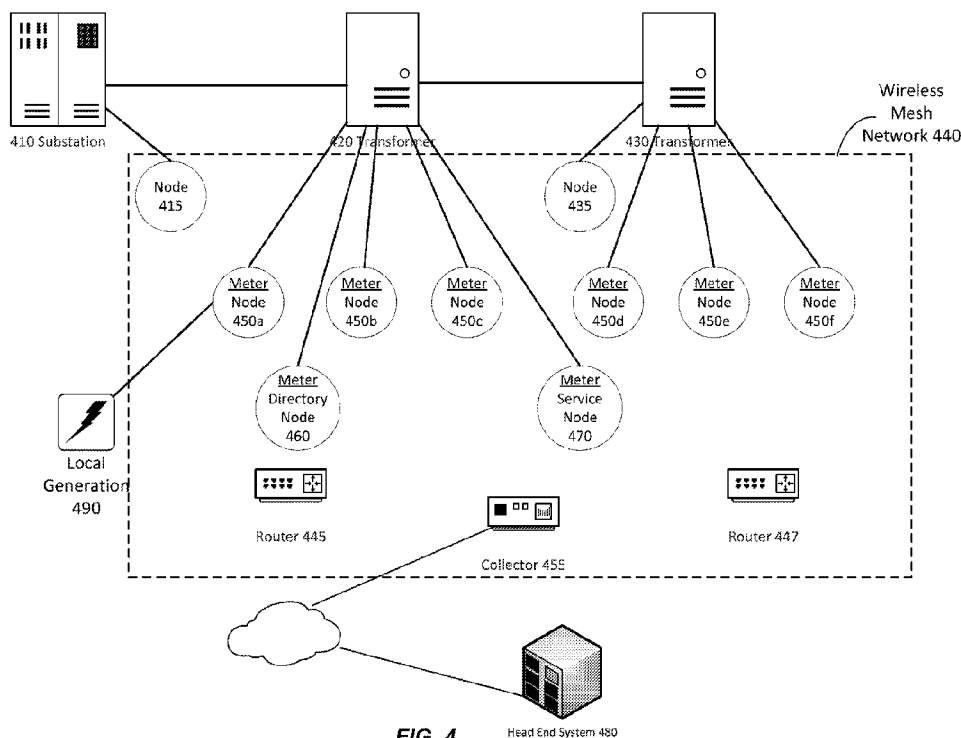
FIG. 4 Head End System 480
