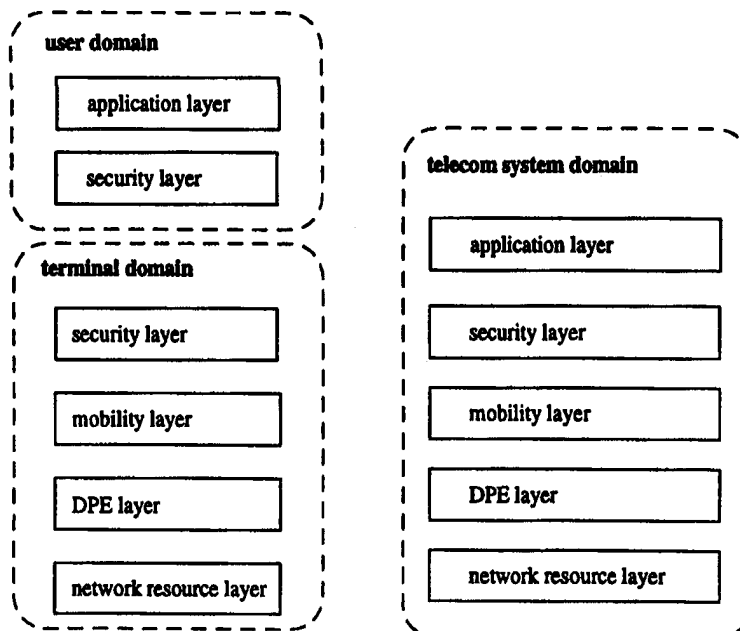
The Functional Separation Architecture supporting mobility
