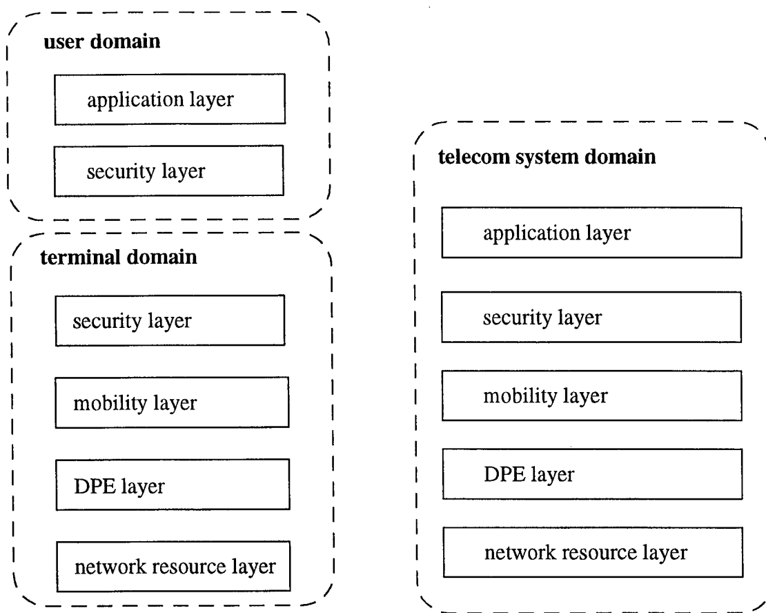
Figure 1 The Functional Separation Architecture supporting mobility
