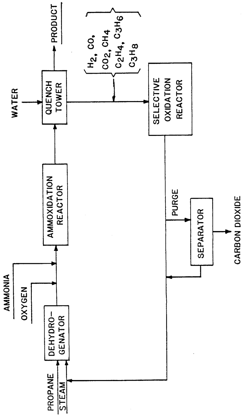
FIG. 2 (PRIOR ART)
