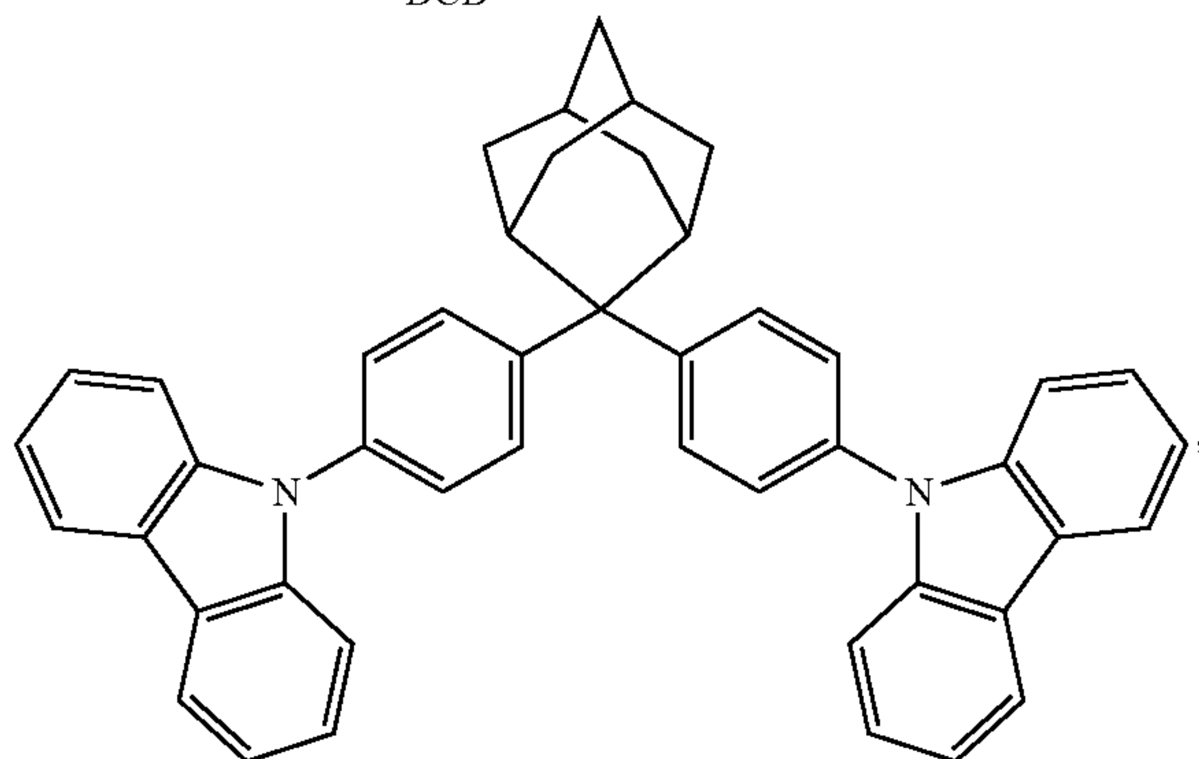
DCz
