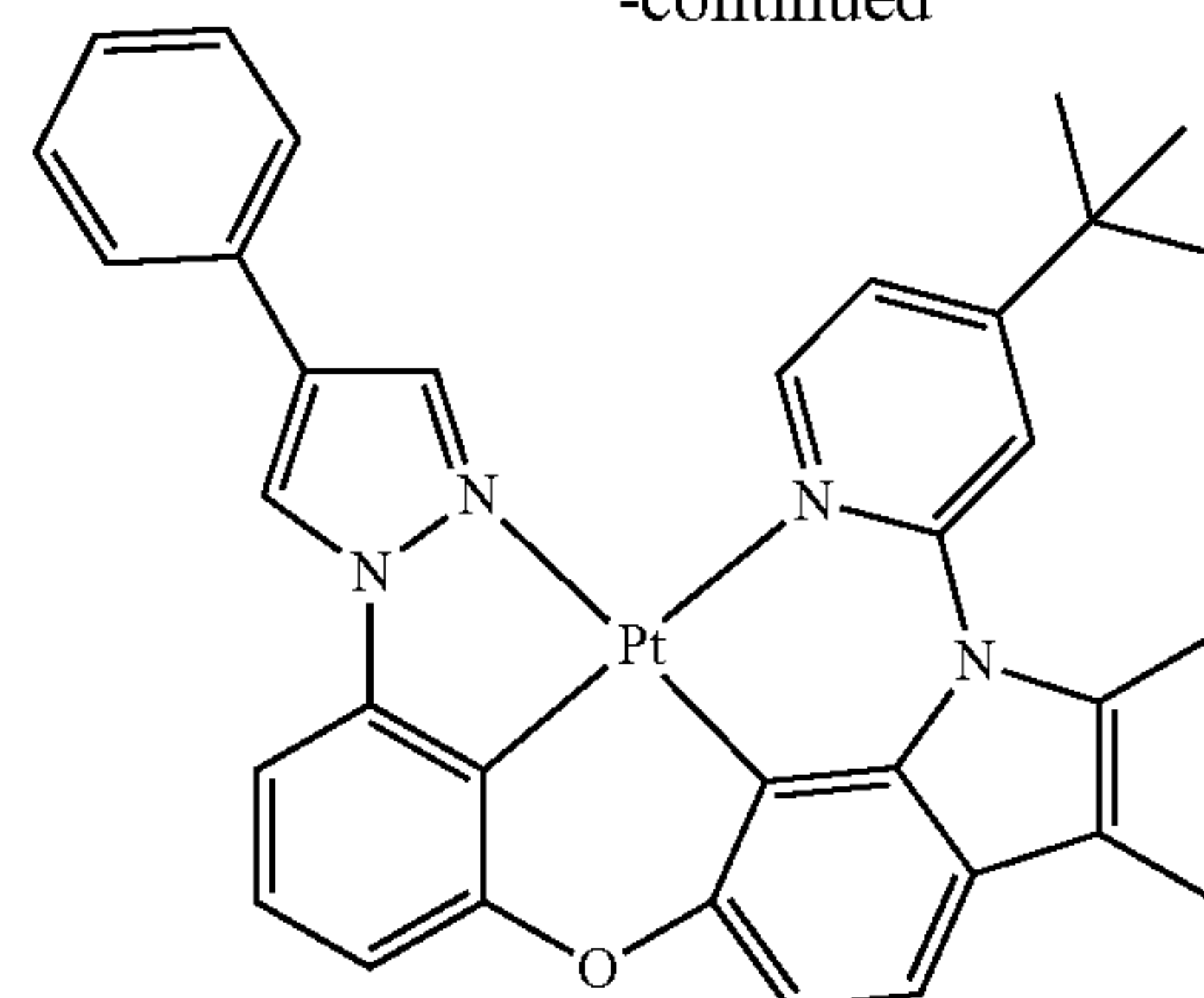
PtON6-tBu
