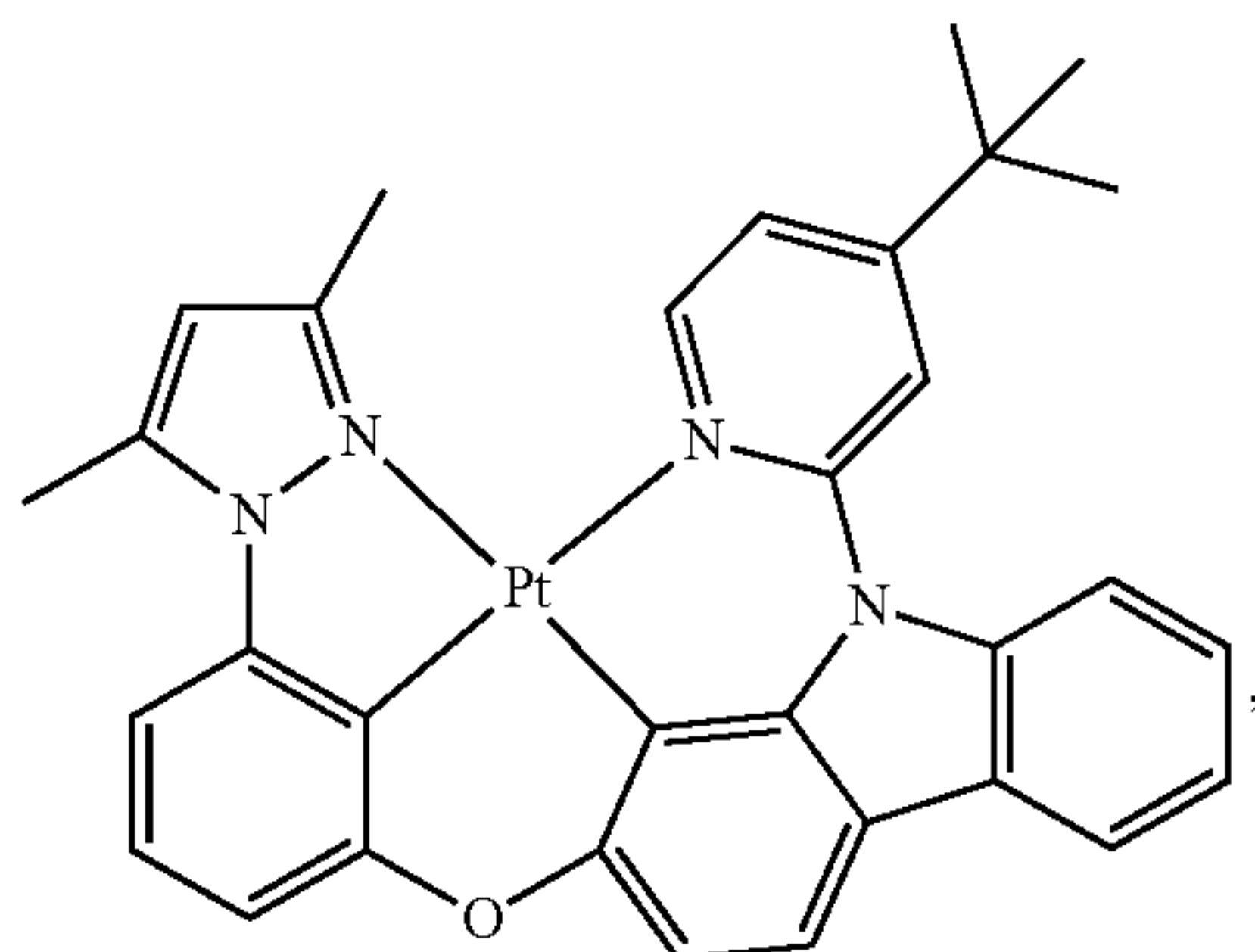
PtON1-tBu
