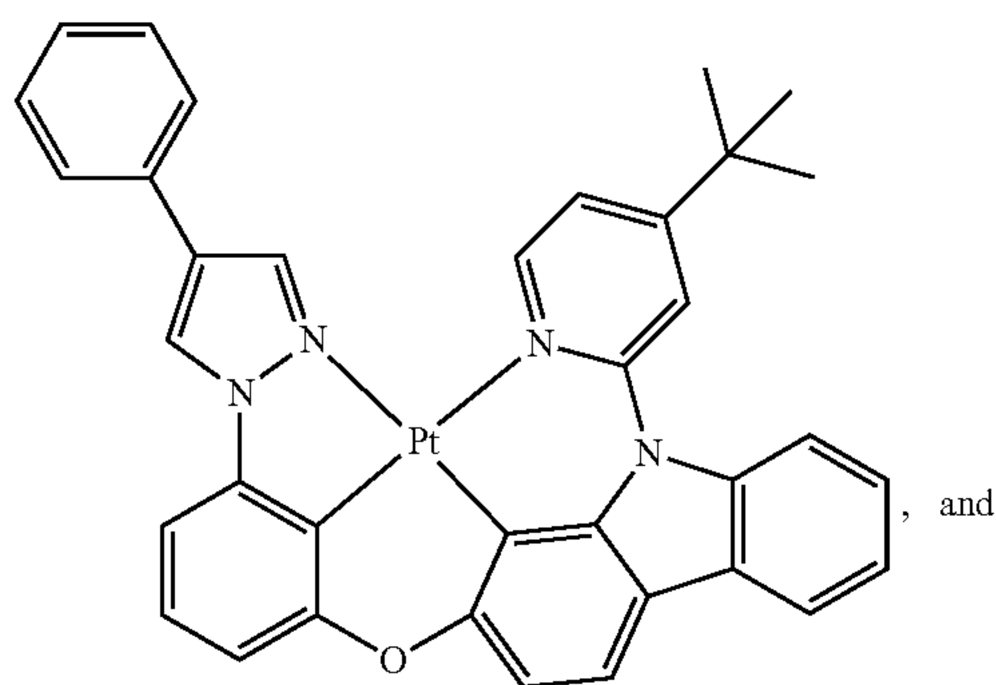
PtON6-tBu
