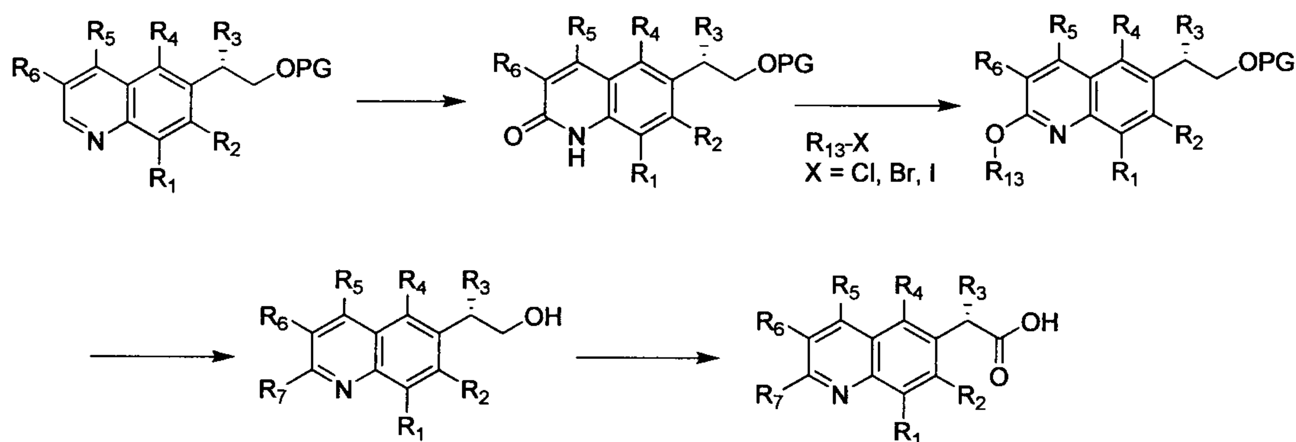
Scheme 3
