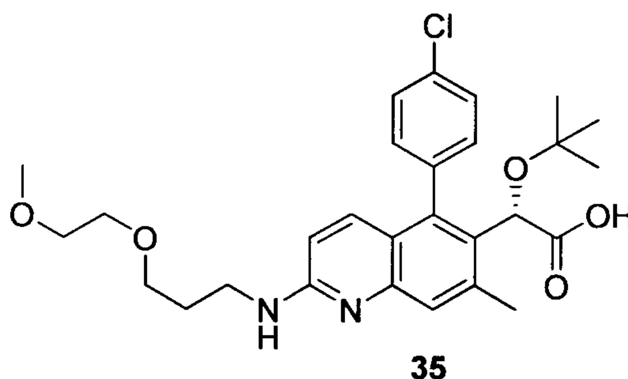
(S)-2-tert-butoxy-2-(5-(4-chlorophenyl)-2-(3-(2-methoxyethoxy)propylamino)-7-methylquinolin-6-yl)acetic acid
