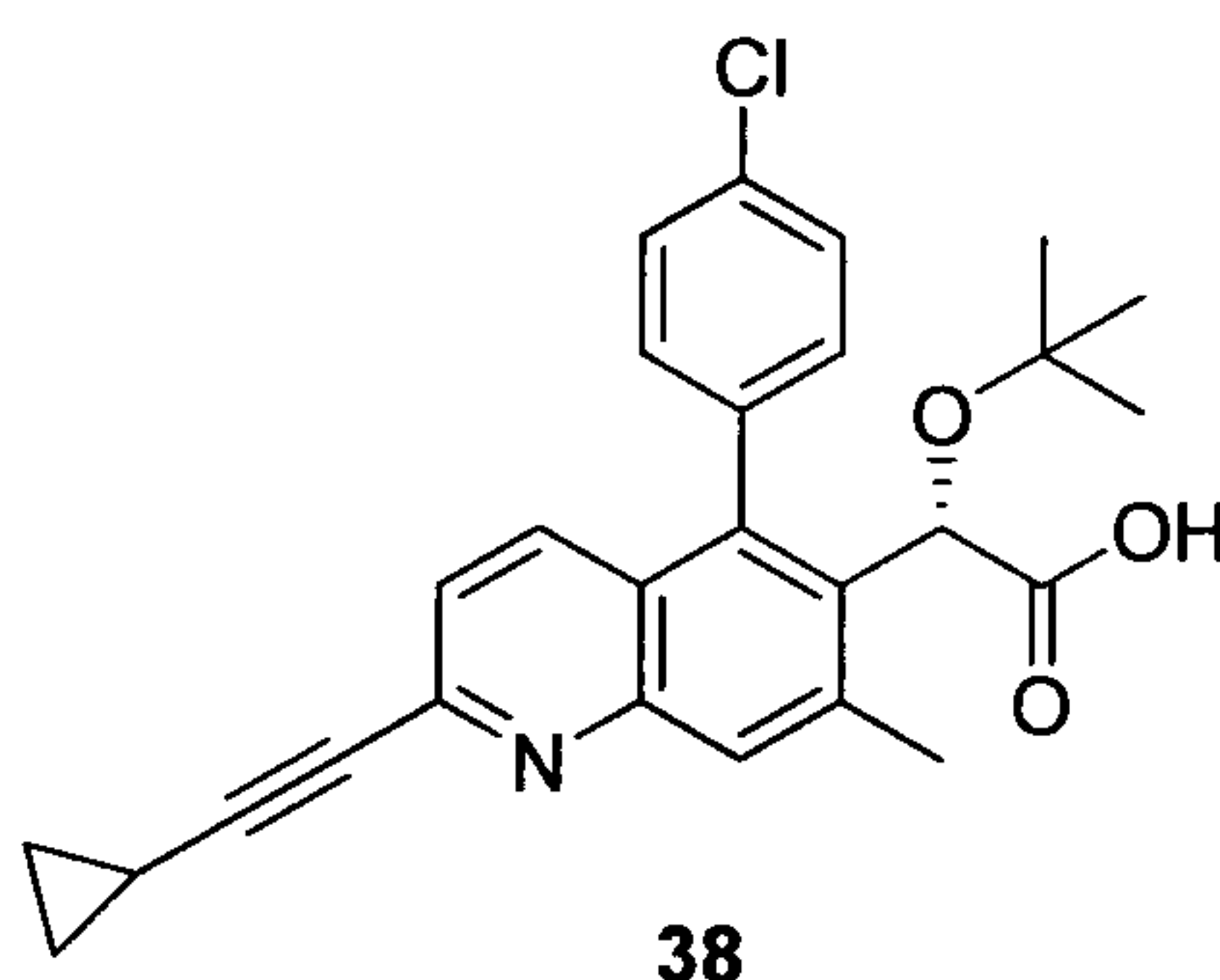
(S)-2-tert-butoxy-2-(5-(4-chlorophenyl)-2-(cyclopropylethynyl)-7-methylquinolin-6-yl)acetic acid
