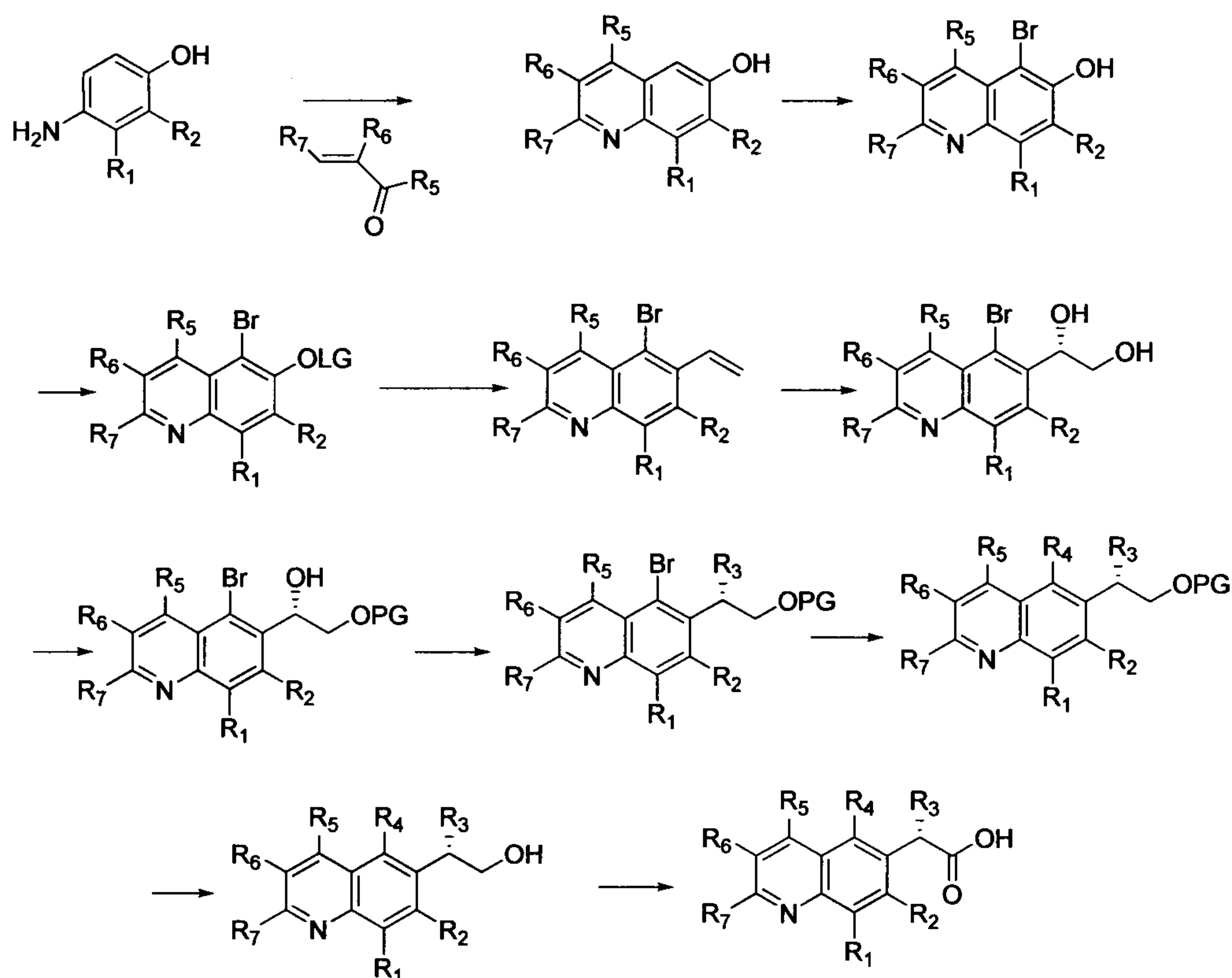
Scheme 1
