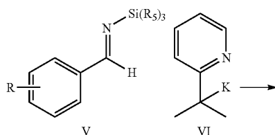
Scheme II
