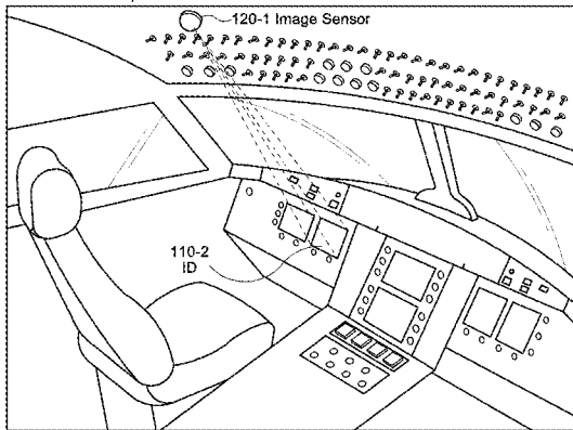
150 Aircraft Cockpit
