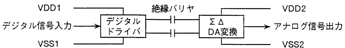
(e) DA変換
