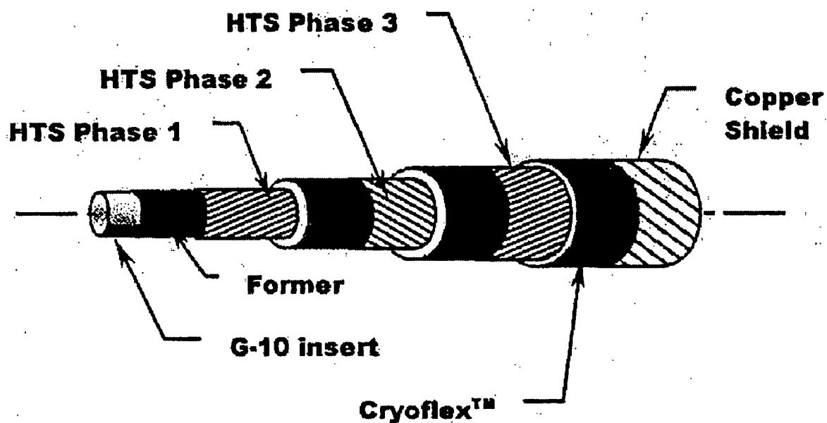
Fig. 2. Schematic of the tri-axial cable.
