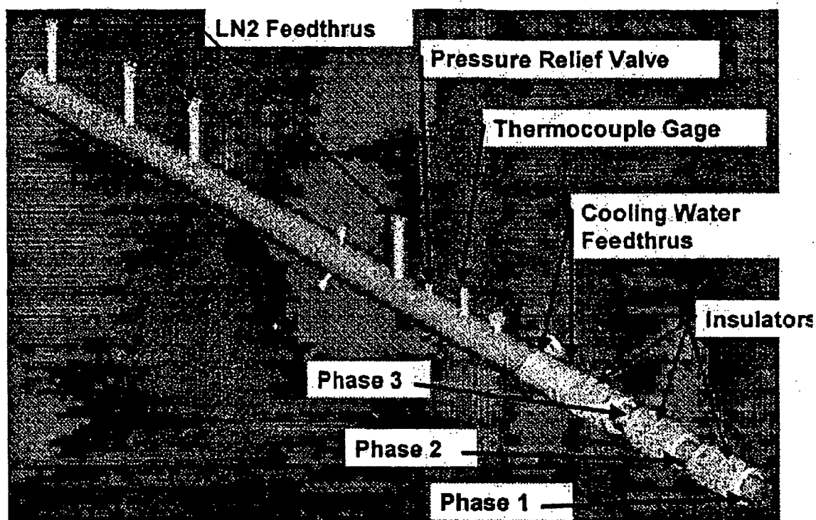
Fig. 6. Rendering of the tri-axial termination.
