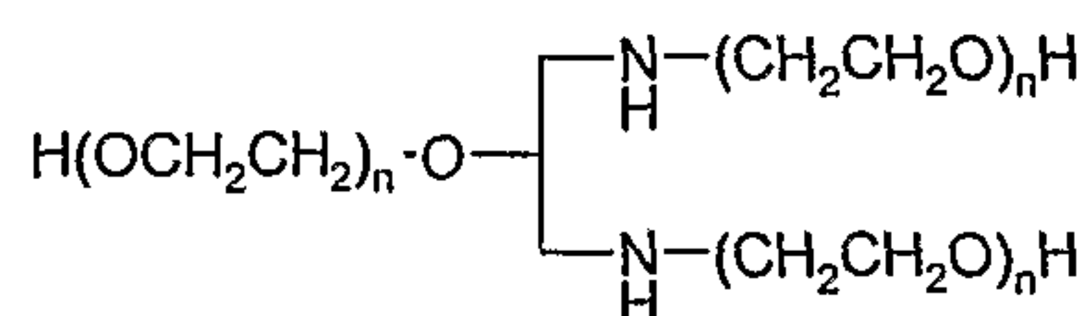
tri-PEG-1,3-diamino-2-hydroxypropane
