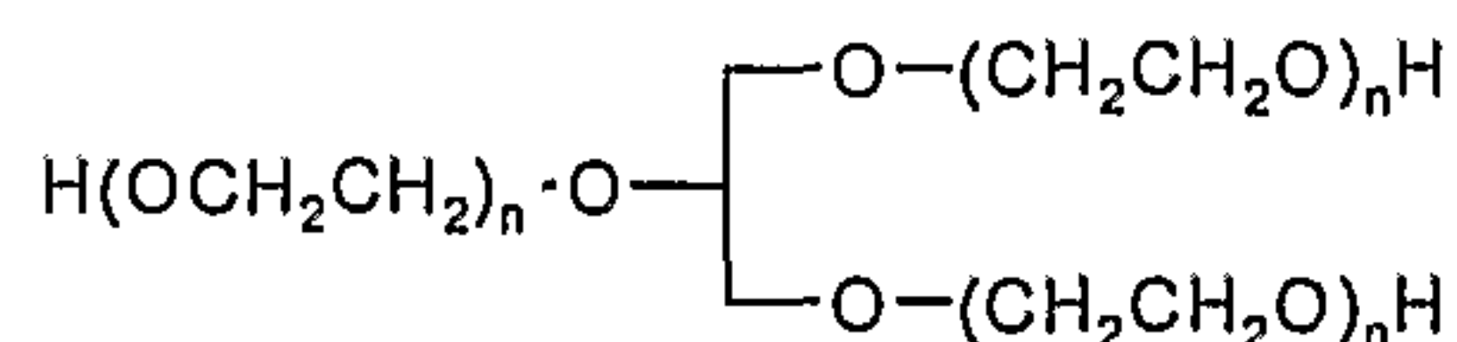
tri-PEG-glycerol
