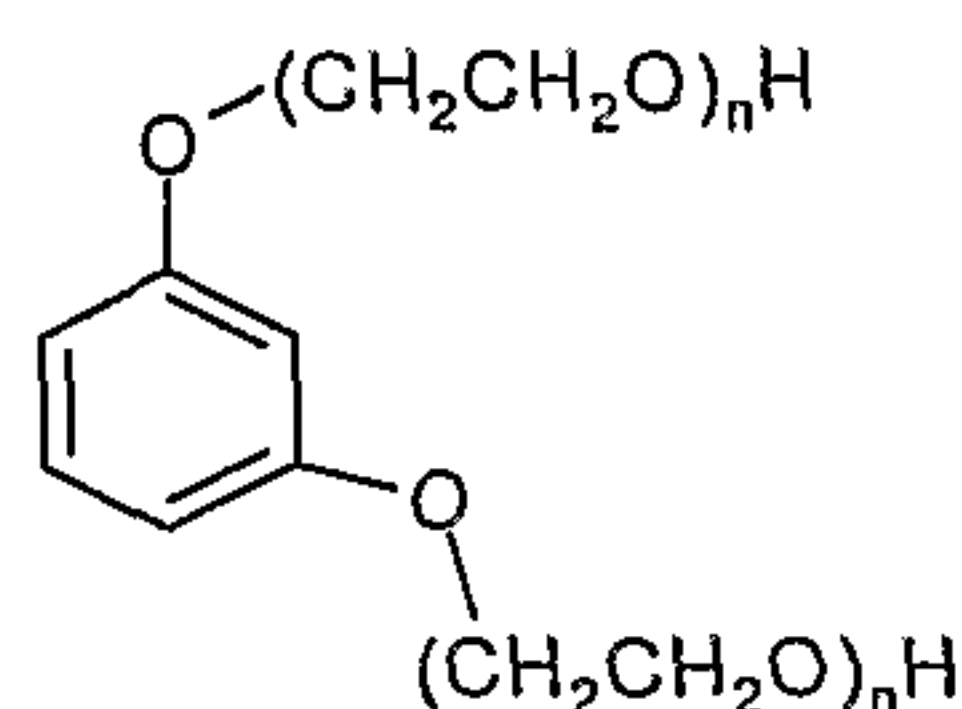
di-PEG resorcinol
