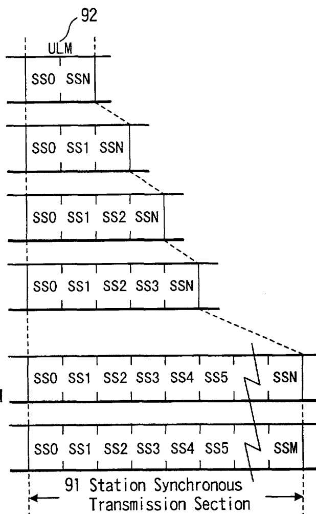
FIG. 9E The Number of Terminal Stations: Maximum-1
