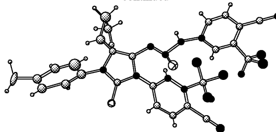
X-ray structure of 35a
