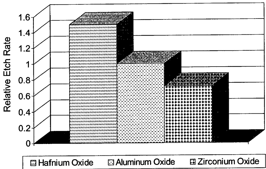
Relative etch rate comparison for HfO 2 , Al 2 O 3 , and ZrO 2 .
